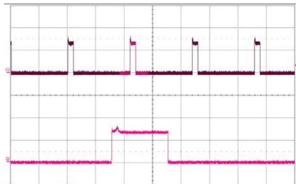
Figure 16. Load current (top trace, 20 A/div., 100 ms/div.) into a 10 m\Omega short circuit during restart, at V_{in} = 48 V. Bottom trace (20 A/div., 10 ms/div.) is an expansion of the on-time portion of the top trace.
