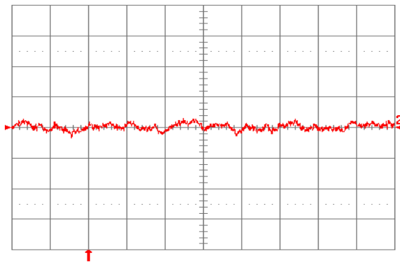
Fig. 5.0V.16: Input reflected ripple current, i_s (10 mA/div.), measured through 10 \mu\text{H} at the source at full rated load current and V_{in} = 24\text{V} . Refer to Fig. 5.0V.14 for test setup. Time scale: 1 \mu\text{s}/\text{div} .
