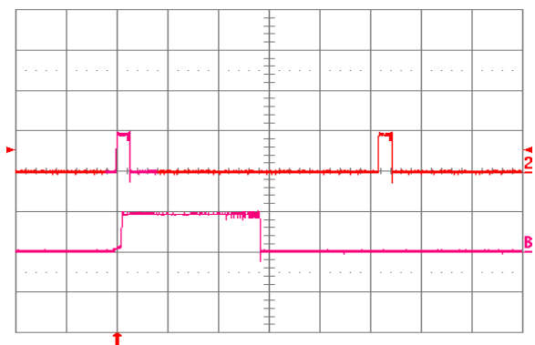
Fig. 2.0V.18: Load current (top trace, 20 \text{A}/\text{div} ., 20 \text{ms}/\text{div} .) into a 10 \text{m}\Omega short circuit during restart, at V_{in} = 24 \text{V} . Bottom trace ( 20 \text{A}/\text{div} ., 2 \text{ms}/\text{div} .) is an expansion of the on-time portion of the top trace.
