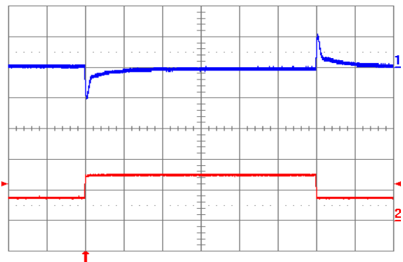
Fig. 1.8V.12: Output voltage response to load current step-change (3.75A – 7.5A – 3.75A) at V in = 24V. Top trace: output voltage (100 mV/div.). Bottom trace: load current (5 A/div.). Current slew rate: 5 A/µs. C o = 450 µF tantalum + 1 µF ceramic. Time scale: 0.2 ms/div.
