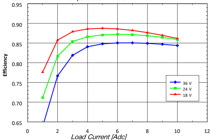
Fig. 5.0V.5: Efficiency vs. load current and input voltage for SQ24T/S10050 converter mounted vertically with air flowing from pin 3 to pin 1 at a rate of 300 LFM (1.5 m/s) and T_a = 25^{\circ}\text{C} .
