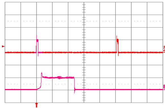
Fig. 2.5V.18: Load current (top trace, 20 \text{ A}/\text{div} ., 20 \text{ ms}/\text{div} .) into a 10 \text{ m}\Omega short circuit during restart, at V_{in} = 24 \text{ V} . Bottom trace ( 20 \text{ A}/\text{div} ., 1 \text{ ms}/\text{div} .) is an expansion of the on-time portion of the top trace.
