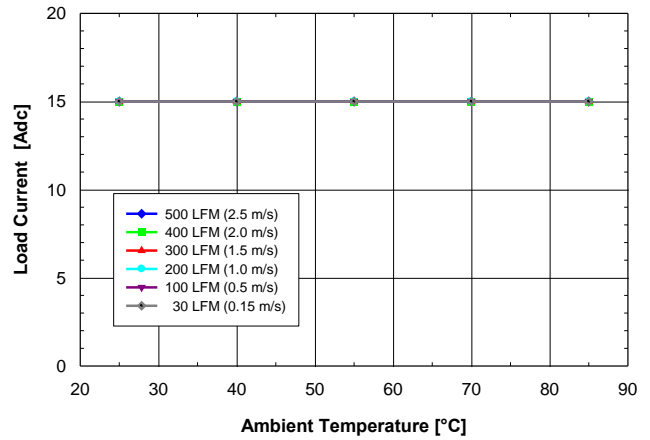
Fig. 1.5V.2: Available load current vs. ambient air temperature and airflow rates for SQ24T15015 converter mounted horizontally with V_{in} = 24V , air flowing from pin 3 to pin 1 and maximum FET temperature \leq 120^{\circ}C .
