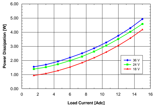
Fig. 1.5V.7: Power dissipation vs. load current and input voltage for SQ24T/S15015 converter mounted vertically with air flowing from pin 3 to pin 1 at a rate of 300 LFM (1.5 m/s) and T a = 25°C.
