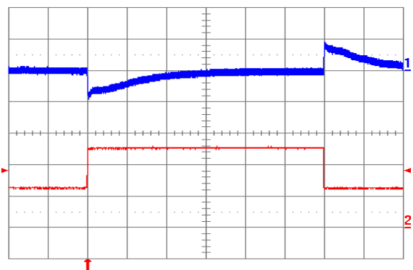
Fig. 5.0V.12: Output voltage response to load current step-change (2.5A - 5A - 2.5A) at Vin = 24V. Top trace: output voltage (100 mV/div.). Bottom trace: load current (2 A/div.). Current slew rate: 5 A/µs. Co = 450 µF tantalum + 1 µF ceramic. Time scale: 0.2 ms/div.
