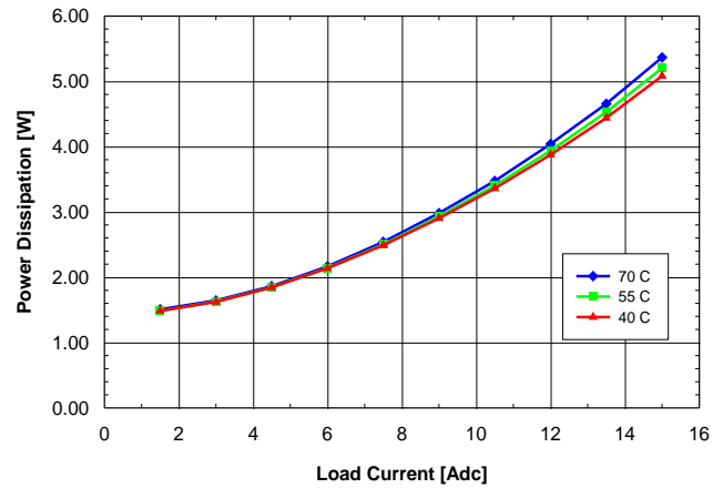
Fig. 2.0V.8: Power dissipation vs. load current and ambient temperature for SQ24T/S15020 converter mounted vertically with V in = 24V and air flowing from pin 3 to pin 1 at a rate of 200 LFM (1.0 m/s).
