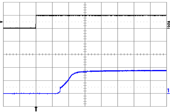
Fig. 1.8V.9: Turn-on transient at full rated load current (resistive) with no output capacitor at V in = 24V, triggered via ON/OFF pin. Top trace: ON/OFF signal (5 V/div.). Bottom trace: output voltage (1 V/div.). Time scale: 1 ms/div.
