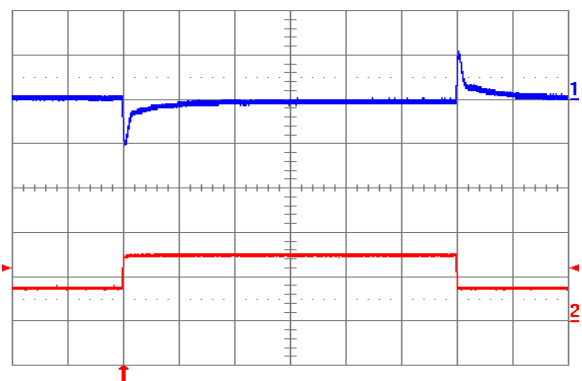
Fig. 1.8V.12: Output voltage response to load current step-change (3.75A – 7.5A – 3.75A) at V in = 24V. Top trace: output voltage (100 mV/div.). Bottom trace: load current (5 A/div.). Current slew rate: 5 A/µs. C o = 450 µF tantalum + 1 µF ceramic. Time scale: 0.2 ms/div.
