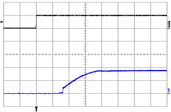
Fig. 1.8V.10: Turn-on transient at full rated load current (resistive) plus 10,000µF at V in = 24V, triggered via ON/OFF pin. Top trace: ON/OFF signal (5 V/div.). Bottom trace: output voltage (1 V/div.). Time scale: 1 ms/div.
