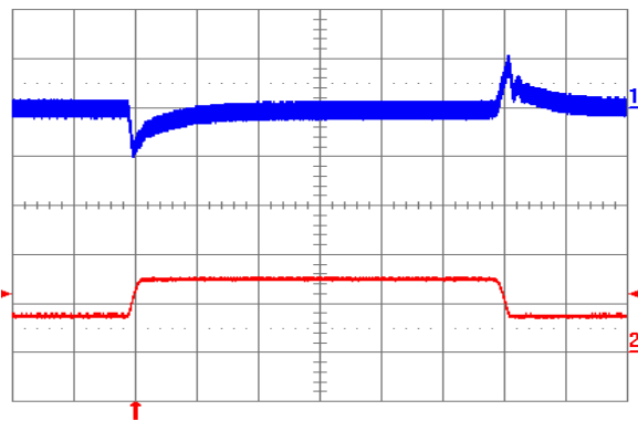
Fig. 2.0V.11: Output voltage response to load current step-change (3.75A – 7.5A – 3.75A) at V in = 24V. Top trace: output voltage (100 mV/div.). Bottom trace: load current (5 A/div.). Current slew rate: 0.1 A/µs. C o = 1 µF ceramic. Time scale: 0.2 ms/div.
