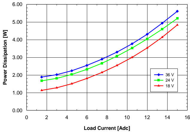
Fig. 2.0V.7: Power dissipation vs. load current and input voltage for SQ24T/S15020 converter mounted vertically with air flowing from pin 3 to pin 1 at a rate of 300 LFM (1.5 m/s) and T a = 25°C.
