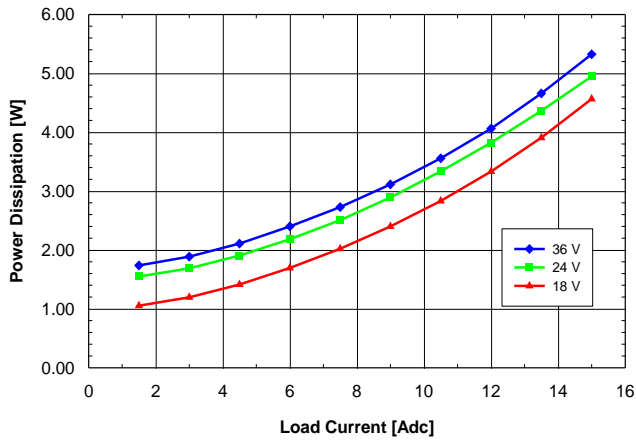
Fig. 1.8V.7: Power dissipation vs. load current and input voltage for SQ24T/S15018 converter mounted vertically with air flowing from pin 3 to pin 1 at a rate of 300 LFM (1.5 m/s) and T a = 25°C.
