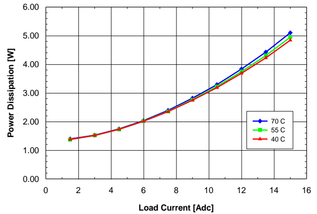
Fig. 1.8V.8: Power dissipation vs. load current and ambient temperature for SQ24T/S15018 converter mounted vertically with V in = 24V and air flowing from pin 3 to pin 1 at a rate of 200 LFM (1.0 m/s).
