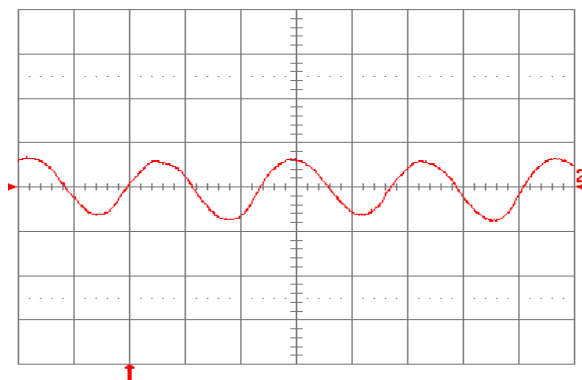
Fig. 5.0V.15: Input reflected ripple current, i_c (100 mA/div.), measured at input terminals at full rated load current and V_{in} = 24\text{V} . Refer to Fig. 5.0V.14 for test setup. Time scale: 1 \mu\text{s}/\text{div} .
