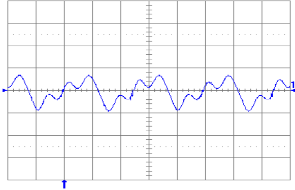
Fig. 2.0V.13: Output voltage ripple (20 mV/div.) at full rated load current into a resistive load with C_o = 10 \mu\text{F} tantalum + 1 \mu\text{F} ceramic and V_{in} = 24 \text{V} . Time scale: 1 \mu\text{s}/\text{div} .
