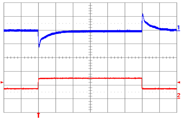
Fig. 2.0V.12: Output voltage response to load current step-change (3.75A – 7.5A – 3.75A) at V in = 24V. Top trace: output voltage (100 mV/div.). Bottom trace: load current (5 A/div.). Current slew rate: 5 A/µs. C o = 450 µF tantalum + 1 µF ceramic. Time scale: 0.2 ms/div.
