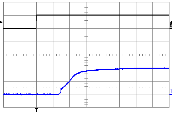
Fig. 2.0V.9: Turn-on transient at full rated load current (resistive) with no output capacitor at V in = 24V, triggered via ON/OFF pin. Top trace: ON/OFF signal (5 V/div.). Bottom trace: output voltage (1 V/div.). Time scale: 1 ms/div.
