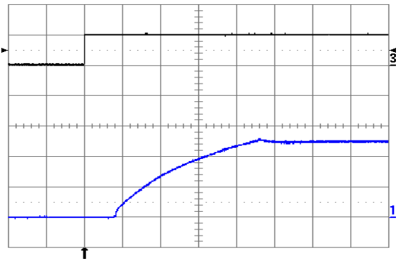
Fig. 5.0V.10: Turn-on transient at full rated load current (resistive) plus 10,000 µF at Vin = 24V, triggered via ON/OFF pin. Top trace: ON/OFF signal (5 V/div.). Bottom trace: output voltage (2 V/div.). Time scale: 2 ms/div.
