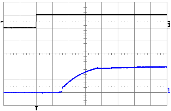
Fig. 2.0V.10: Turn-on transient at full rated load current (resistive) plus 10,000µF at V in = 24V, triggered via ON/OFF pin. Top trace: ON/OFF signal (5 V/div.). Bottom trace: output voltage (1 V/div.). Time scale: 1 ms/div.
