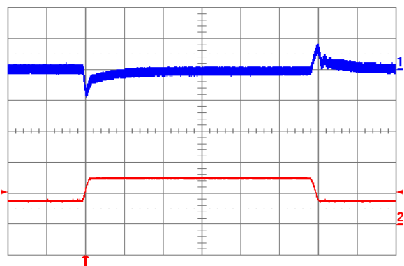
Fig. 1.8V.11: Output voltage response to load current step-change (3.75A – 7.5A – 3.75A) at V in = 24V. Top trace: output voltage (100 mV/div.). Bottom trace: load current (5 A/div.). Current slew rate: 0.1 A/µs. C o = 1 µF ceramic. Time scale: 0.2 ms/div.
