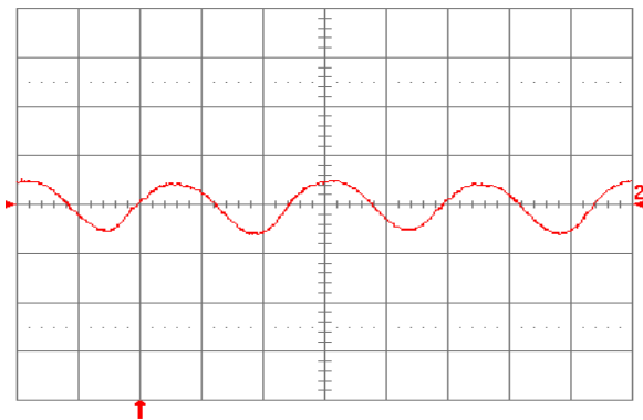
Fig. 2.0V.15: Input reflected ripple current, i_c (100 mA/div.), measured at input terminals at full rated load current and V_{in} = 24\text{V} . Refer to Fig. 2.0V.14 for test setup. Time scale: 1 \mu\text{s}/\text{div} .
