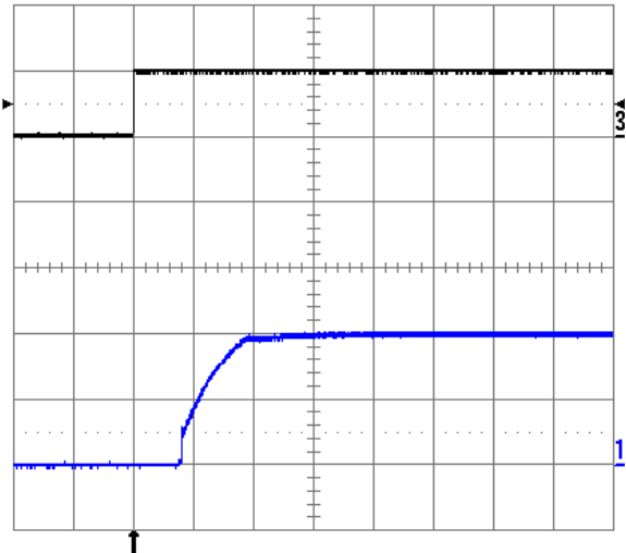
Fig. 2.0V.10: Turn-on transient at full rated load current (resistive) plus 10,000\mu F at V_{in} = 48V , triggered via ON/OFF pin. Top trace: ON/OFF signal (5V/div.). Bottom trace: output voltage (1V/div.). Time scale: 2ms/div.
