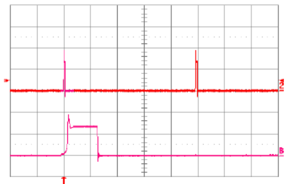
Fig. 5.0V.18: Load current (top trace, 10\text{A}/\text{div} ., 20\text{ms}/\text{div} .) into a 10\text{m}\Omega short circuit during restart, at V_{in} = 48\text{V} . Bottom trace ( 10\text{A}/\text{div} ., 1\text{ms}/\text{div} .) is an expansion of the on-time portion of the top trace.
