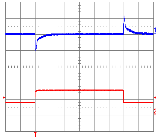
Fig. 2.0V.12: Output voltage response to load current step-change ( 3.75 A - 7.5 A - 3.75 A ) at V_{in} = 48V . Top trace: output voltage (100 mV/div.). Bottom trace: load current (5A/div.). Current slew rate: 5 A/\mu s . C_o = 450 \mu F tantalum + 1 \mu F ceramic. Time scale: 0.2 ms/div.
