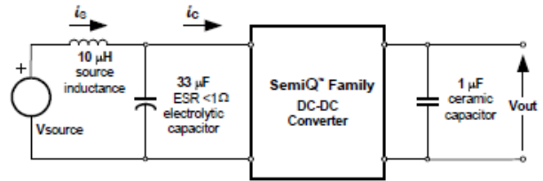
Fig. 1.8V.14: Test Setup for measuring input reflected ripple currents, i_c and i_s
