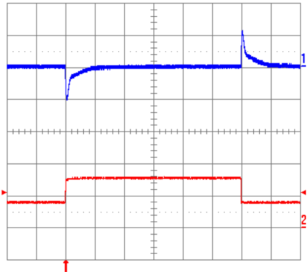
Fig. 2.0V.12: Output voltage response to load current step-change (3.75 A – 7.5 A – 3.75 A) at V_{in} = 48V . Top trace: output voltage (100 mV/div.). Bottom trace: load current (5A/div.). Current slew rate: 5 A/ \mu s . C_o = 450\mu F tantalum + 1 \mu F ceramic. Time scale: 0.2 ms/div.
