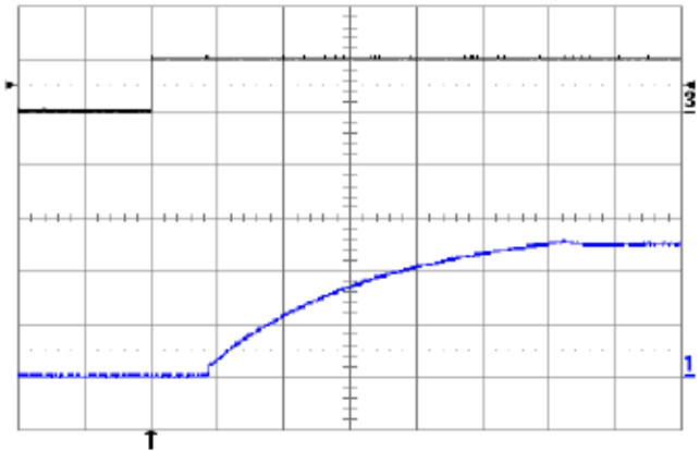
Fig. 5.0V.10: Turn-on transient at full rated load current (resistive) plus 10,000\mu F at V_{in} = 48V , triggered via ON/OFF pin. Top trace: ON/OFF signal (5V/div.). Bottom trace: output voltage (2V/div.). Time scale: 5ms/div.
