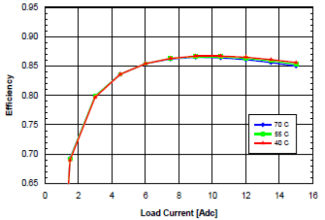
Fig. 1.8V.6: Efficiency vs. load current and ambient temperature for SQ48T/S15018 converter mounted vertically with V_{in} = 48\text{V} and air flowing from pin 3 to pin 1 at a rate of 200LFM (1.0 m/s).
