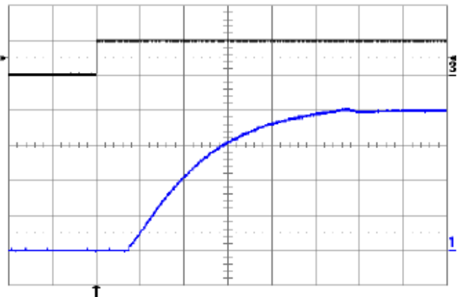
Fig. 8.0V.8: Turn-on transient at full rated load current (resistive) plus 2,200 \mu\text{F} at V_{in} = 48\text{V} , triggered via ON/OFF pin. Top trace: ON/OFF signal (5V/div.). Bottom trace: output voltage (2V/div.). Time scale: 2ms/div.
