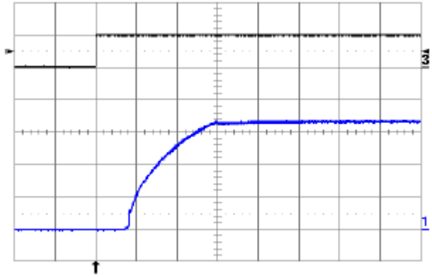
Fig. 3.3V.10: Turn-on transient at full rated load current (resistive) plus 10,000 \mu F at V_{in} = 48V , triggered via ON/OFF pin. Top trace: ON/OFF signal (5V/div.). Bottom trace: output voltage (1V/div.). Time scale: 2ms/div.
