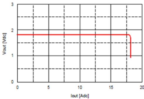
Fig. 1.8V.17: Output voltage vs. load current showing current limit point and converter shutdown point. Input voltage has almost no effect on current limit characteristic.
