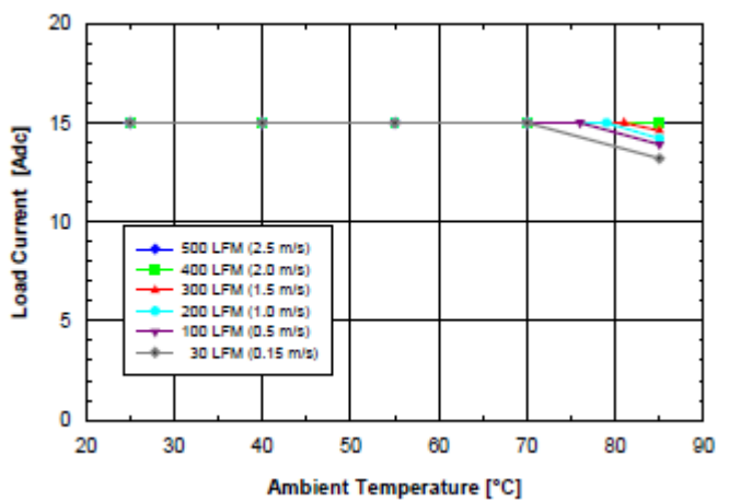
Figure 1.8V.4 Available load current vs. ambient air temperature and airflow rates for SQ48S15018 converter with D height pins mounted horizontally with V_{in} = 48V , air flowing from pin 3 to pin 1, and maximum FET temperature \leq 120^{\circ}C .
