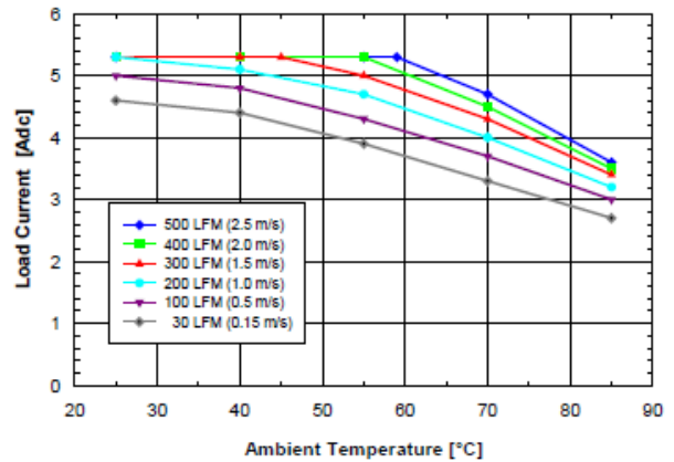
Figure 8.0V.2 Available load current vs. ambient air temperature and airflow rates for SQ48T05080 converter with D height pins mounted horizontally with V_{in} = 48V , air flowing from pin 3 to pin 1, and maximum FET temperature \leq 120^{\circ}C .
