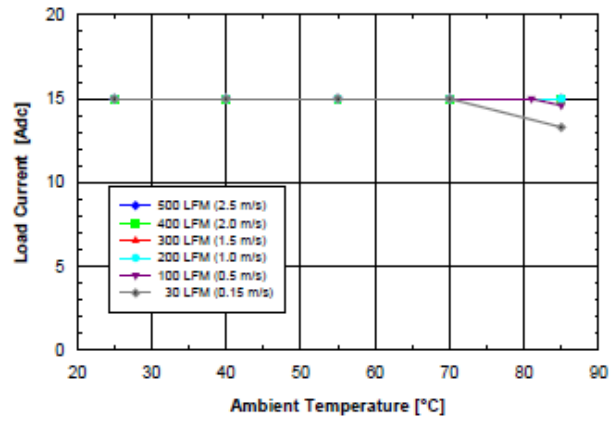
Figure 1.5V.2 Available load current vs. ambient air temperature and airflow rates for SQ48T15015 converter with D height pins mounted horizontally with V_{in} = 48V , air flowing from pin 3 to pin 1, and maximum FET temperature \leq 120^{\circ}C .
