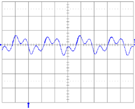
Fig. 2.5V.13: Output voltage ripple (20 mV/div.) at full rated load current into a resistive load with C_o = 10\mu\text{F} tantalum + 1\mu\text{F} ceramic and V_{in} = 48\text{V} . Time scale: 1\mu\text{s}/\text{div} .
