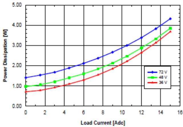
Fig. 1.2V.7: Power dissipation vs. load current and input voltage for SQ48T/S15012 converter mounted vertically with air flowing from pin 3 to pin 1 at a rate of 300 LFM (1.5 m/s) and Ta = 25°C.
