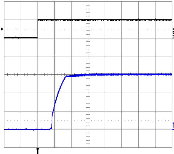
Fig. 1.5V.10: Turn-on transient at full rated load current (resistive) plus 10,000 \mu F at V_{in} = 48V , triggered via ON/OFF pin. Top trace: ON/OFF signal (5V/div.). Bottom trace: output voltage (0.5V/div.). Time scale: 2ms/div.
