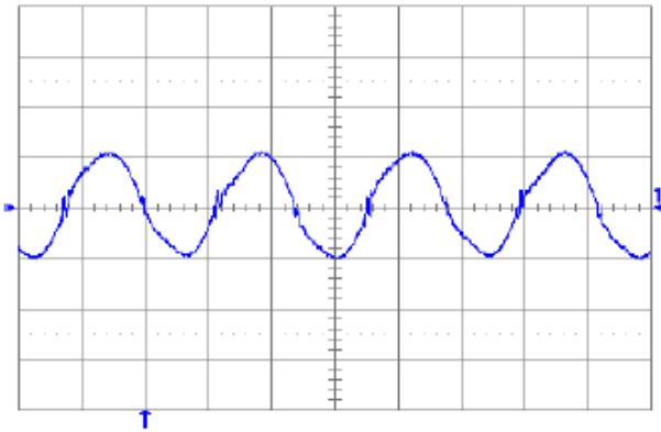
Fig. 5.0V.13: Output voltage ripple (20 mV/div.) at full rated load current into a resistive load with C_o = 10\mu\text{F} tantalum + 1\mu\text{F} ceramic and V_{in} = 48\text{V} . Time scale: 1\mu\text{s}/\text{div} .
