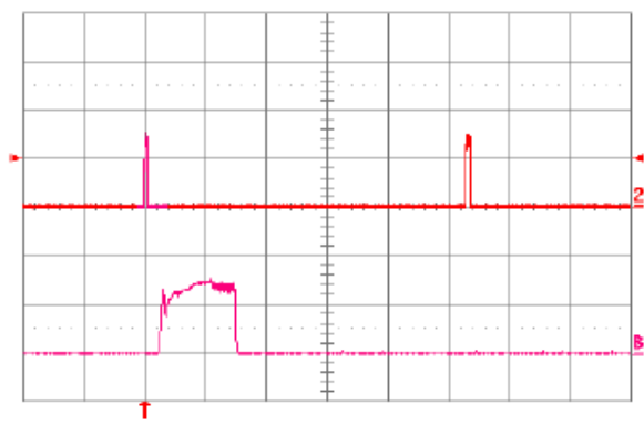
Fig. 8.0V.16: Load current (top trace, 5A/div., 20 ms/div.) into a 10 m \Omega short circuit during restart, at V_{in} = 48V . Bottom trace (5A/div., 1ms/div.) is an expansion of the on-time portion of the top trace.
