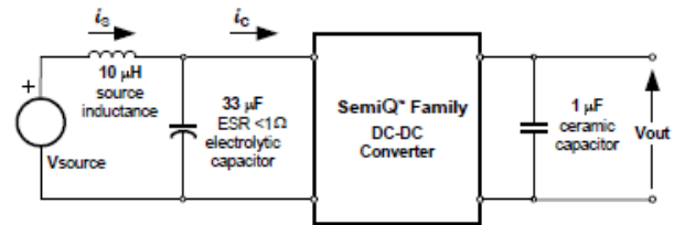
Fig. 6.0V.12: Test Setup for measuring input reflected ripple currents, i_c and i_s
