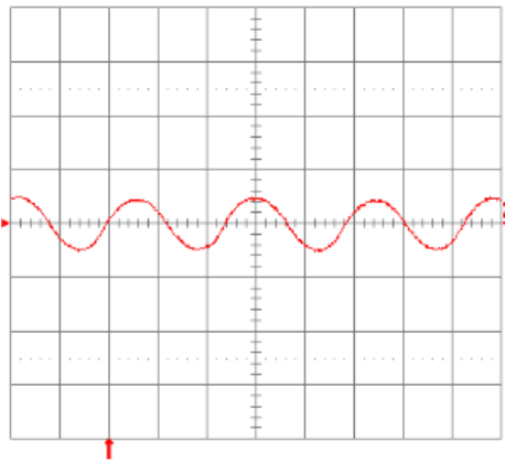
Fig. 2.5V.13: Output voltage ripple (20 mV/div.) at full rated load current into a resistive load with C_o = 10\mu\text{F} tantalum + 1\mu\text{F} ceramic and V_{in} = 48\text{V} . Time scale: 1\mu\text{s}/\text{div} .
