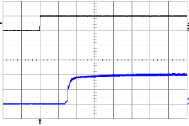
Fig. 1.0V.9: Turn-on transient at full rated load current (resistive) with no output capacitor at V_{in} = 48V , triggered via ON/OFF pin. Top trace: ON/OFF signal (5V/div.). Bottom trace: output voltage (0.5V/div.). Time scale: 2ms/div.
