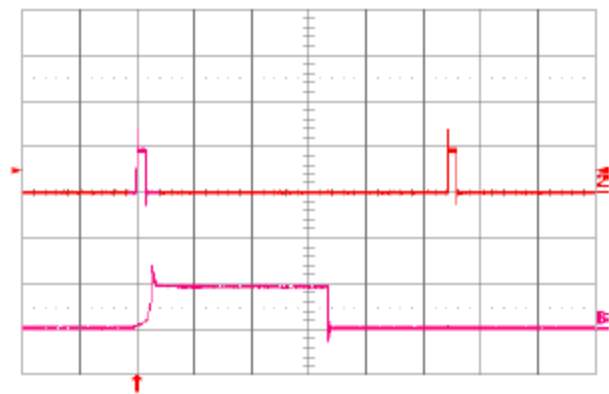
Fig. 1.0V.18: Load current (top trace, 20A/div., 20 ms/div.) into a 10 m \Omega short circuit during restart, at V_{in} = 48\text{V} . Bottom trace (20A/div., 1ms/div.) is an expansion of the on-time portion of the top trace.
