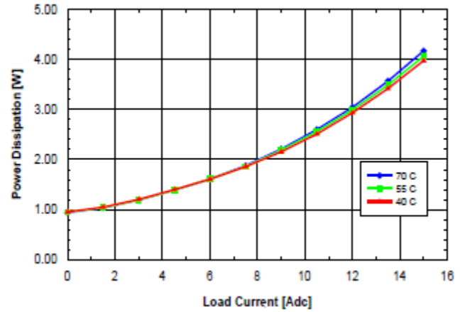
Fig. 1.2V.8: Power dissipation vs. load current and ambient temperature for SQ48T/S15012 converter mounted vertically with Vin = 48V and air flowing from pin 3 to pin 1 at a rate of 200LFM (1.0m/s).
