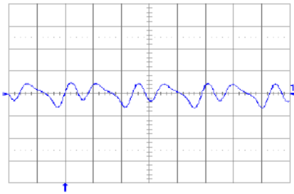
Fig. 1.0V.13: Output voltage ripple (20 mV/div.) at full rated load current into a resistive load with C_o = 10\mu\text{F} tantalum + 1 \mu\text{F} ceramic and V_{in} = 48\text{V} . Time scale: 1 \mu\text{s}/\text{div} .
