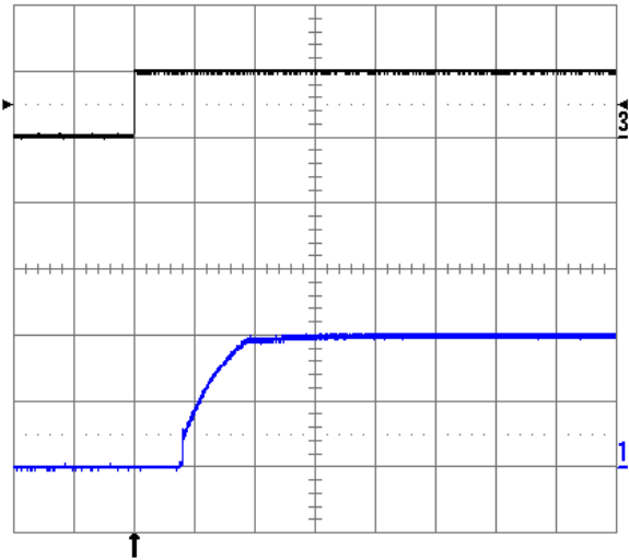
Fig. 2.0V.10: Turn-on transient at full rated load current (resistive) plus 10,000 \mu F at V_{in} = 48V , triggered via ON/OFF pin. Top trace: ON/OFF signal (5V/div.). Bottom trace: output voltage (1V/div.). Time scale: 2ms/div.
