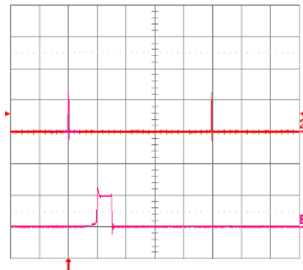
Fig. 2.5V.18: Load current (top trace, 20\text{A}/\text{div} ., 20\text{ms}/\text{div} .) into a 10\text{m}\Omega short circuit during restart, at V_{in} = 48\text{V} . Bottom trace ( 20\text{A}/\text{div} ., 1\text{ms}/\text{div} .) is an expansion of the on-time portion of the top trace.
