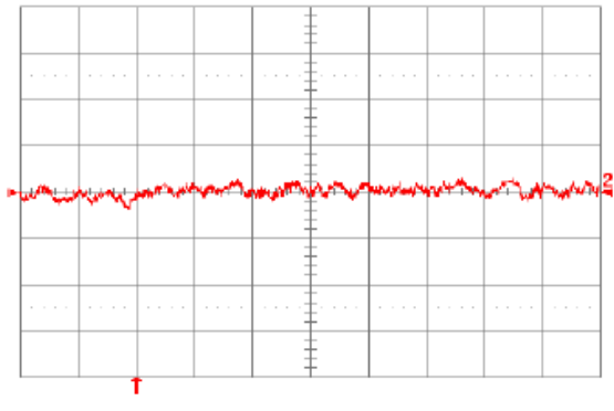
Fig. 8.0V.14: Input reflected ripple current, i_s (10 mA/div.), measured through 10 \mu H at the source at full rated full rated load current and V_{in} = 48V . Refer to Fig. 8.0V.14 for test setup. Time scale: 1 \mu s/div.
