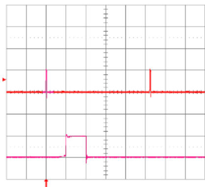
Fig. 1.5V.18: Load current (top trace, 20\text{A}/\text{div} ., 20\text{ms}/\text{div} .) into a 10\text{m}\Omega short circuit during restart, at V_{in} = 48\text{V} . Bottom trace ( 20\text{A}/\text{div} ., 1\text{ms}/\text{div} .) is an expansion of the on-time portion of the top trace.
