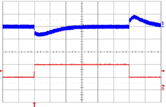
Fig. 6.0V.10: Output voltage response to load current step-change (2 A – 4 A – 2 A) at V_{in} = 48V . Top trace: output voltage (100 mV/div.). Bottom trace: load current (2A/div.). Current slew rate: 5 A/\mu s . C_o = 450\mu F tantalum + 1\mu F ceramic. Time scale: 0.2 ms/div.
