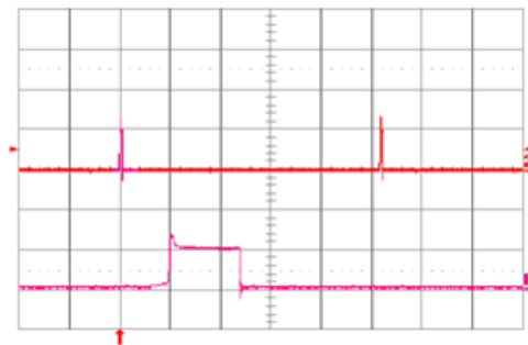
Fig. 1.2V.16: Input reflected ripple current, i_s (10 mA/div.), measured through 10\mu\text{H} at the source at full rated full rated load current and V_{in} = 48\text{V} . Refer to Fig. 1.2V.14 for test setup. Time scale: 1\mu\text{s}/\text{div} .
