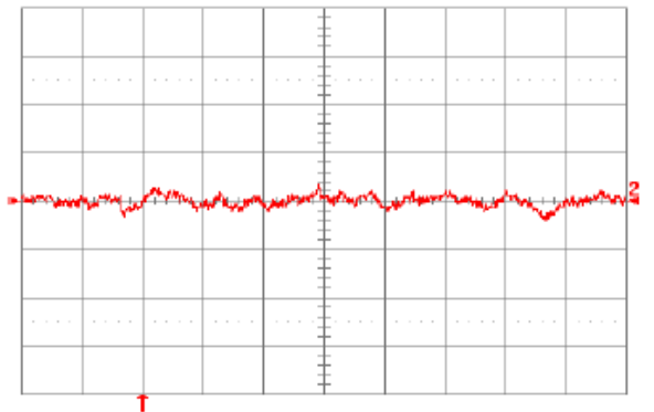
Fig. 5.0V.16: Input reflected ripple current, i_s (10 mA/div.), measured through 10\mu\text{H} at the source at full rated full rated load current and V_{in} = 48\text{V} . Refer to Fig. 5.0V.14 for test setup. Time scale: 1\mu\text{s}/\text{div} .
