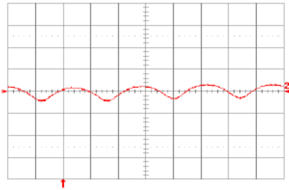
Fig. 1.0V.15: Input reflected ripple current, i_c (100 mA/div.), measured at input terminals at full rated load current and V_{in} = 48\text{V} . Refer to Fig. 1.0V.14 for test setup. Time scale: 1 \mu\text{s}/\text{div} .
