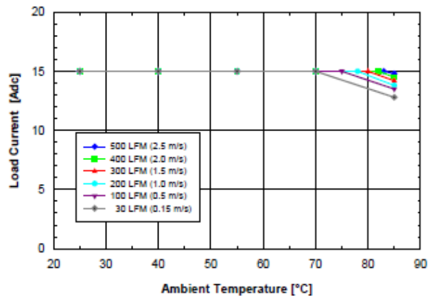
Figure 2.0V.4 Available load current vs. ambient air temperature and airflow rates for SQ48S15020 converter with D height pins mounted horizontally with V_{in} = 48V , air flowing from pin 3 to pin 1, and maximum FET temperature \leq 120^{\circ}C .
