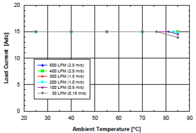
Figure 1.5V.4 Available load current vs. ambient air temperature and airflow rates for SQ48S15015 converter with D height pins mounted horizontally with V_{in} = 48V , air flowing from pin 3 to pin 1, and maximum FET temperature \leq 120^{\circ}C .
