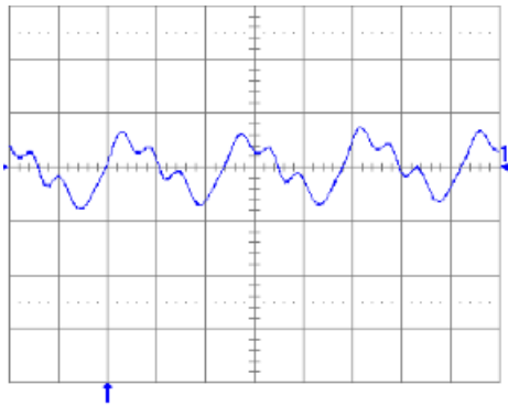
Fig. 3.3V.13: Output voltage ripple (20 mV/div.) at full rated load current into a resistive load with C_o = 10\mu\text{F} tantalum + 1\mu\text{F} ceramic and V_{in} = 48\text{V} . Time scale: 1\mu\text{s}/\text{div} .
