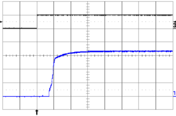
Fig. 3.3V.9: Turn-on transient at full rated load current (resistive) with no output capacitor at V_{in} = 48V , triggered via ON/OFF pin. Top trace: ON/OFF signal (5V/div.). Bottom trace: output voltage (2V/div.). Time scale: 2ms/div.
