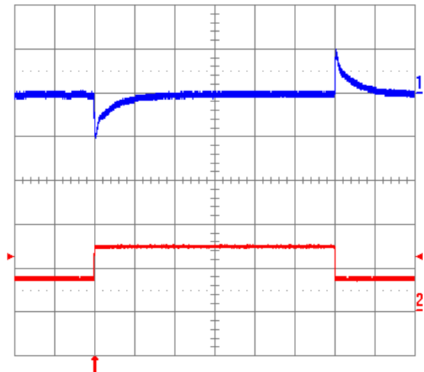
Fig. 3.3V.12: Output voltage response to load current step-change (3.75 A - 7.5 A - 3.75 A) at V_{in} = 48V . Top trace: output voltage (100 mV/div.). Bottom trace: load current (5A/div.). Current slew rate: 5 A/ \mu s . C_o = 450\mu F tantalum + 1 \mu F ceramic. Time scale: 0.2 ms/div.
