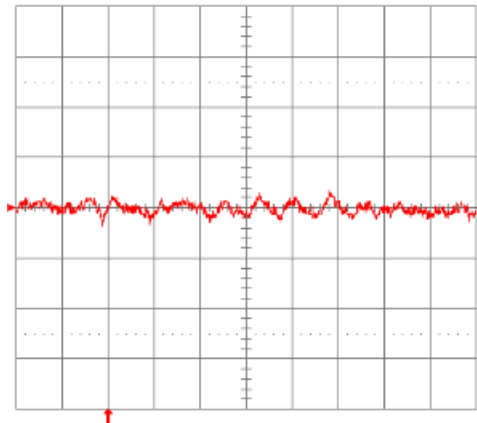
Fig. 3.3V.16: Input reflected ripple current, i_s (10 mA/div.), measured through 10\mu\text{H} at the source at full rated full rated load current and V_{in} = 48\text{V} . Refer to Fig. 3.3V.14 for test setup. Time scale: 1\mu\text{s}/\text{div} .
