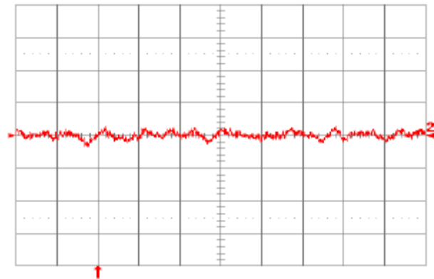
Fig. 1.0V.16: Input reflected ripple current, i_s (10 mA/div.), measured through 10 \mu\text{H} at the source at full rated full rated load current and V_{in} = 48\text{V} . Refer to Fig. 1.0V.14 for test setup. Time scale: 1 \mu\text{s}/\text{div} .
