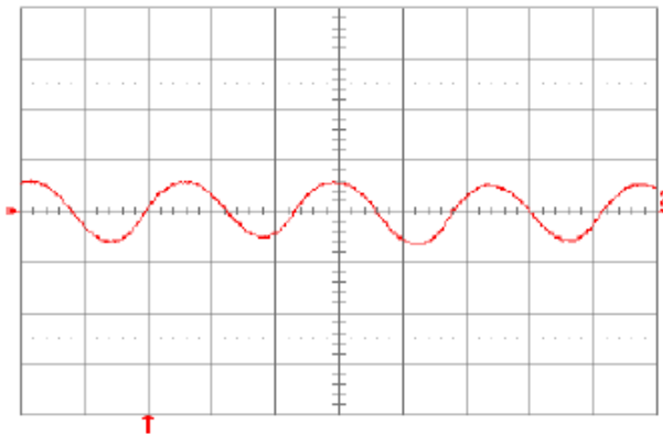
Fig. 5.0V.15: Input reflected ripple current, i_c (100 mA/div.), measured at input terminals at full rated load current and V_{in} = 48\text{V} . Refer to Fig. 5.0V.14 for test setup. Time scale: 1\mu\text{s}/\text{div} .
