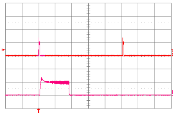
Fig. 12V.16: Load current (top trace, 5A/div., 20 ms/div.) into a 10\ m\Omega short circuit during restart, at V_{in} = 48V . Bottom trace (5A/div., 1ms/div.) is an expansion of the on-time portion of the top trace.
