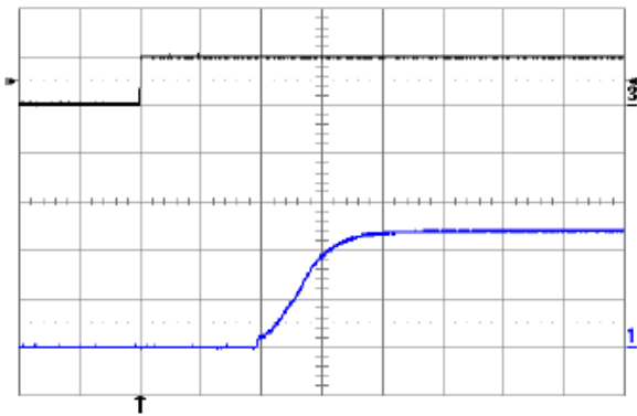
Fig. 12V.7: Turn-on transient at full rated load current (resistive) with no output capacitor at V_{in} = 48\text{V} , triggered via ON/OFF pin. Top trace: ON/OFF signal (5V/div.). Bottom trace: output voltage (5V/div.). Time scale: 1ms/div.
