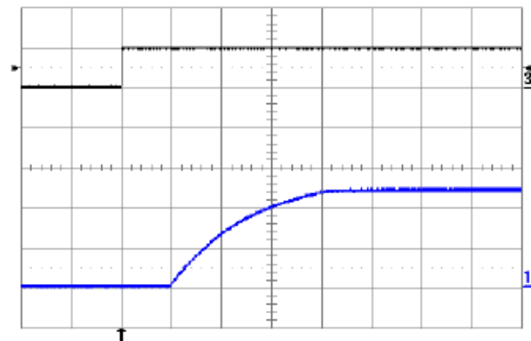
Fig. 12V.8: Turn-on transient at full rated load current (resistive) plus 1,000 µF at V_{in} = 48\text{V} , triggered via ON/OFF pin. Top trace: ON/OFF signal (5V/div.). Bottom trace: output voltage (5V/div.). Time scale: 2ms/div.
