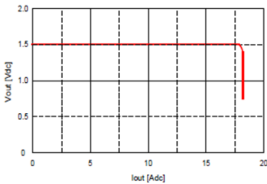
Fig. 1.5V.17: Output voltage vs. load current showing current limit point and converter shutdown point. Input voltage has almost no effect on current limit characteristic.
