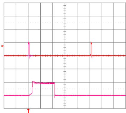
Fig. 3.3V.18: Load current (top trace, 10A/div., 20 ms/div.) into a 10\text{m}\Omega short circuit during restart, at V_{in} = 48\text{V} . Bottom trace (20A/div., 1ns/div.) is an expansion of the on-time portion of the top trace.
