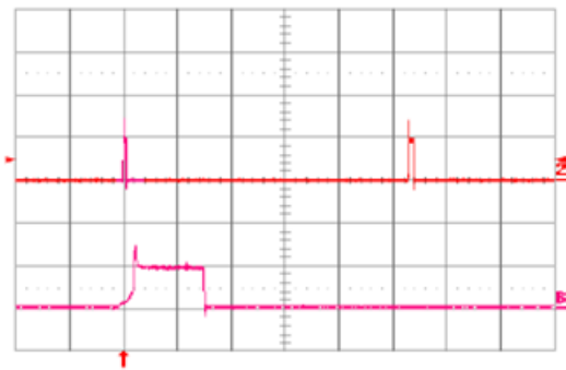
Fig. 1.8V.18: Load current (top trace, 20\text{A}/\text{div} ., 20\text{ms}/\text{div} .) into a 10\text{m}\Omega short circuit during restart, at V_{in} = 48\text{V} . Bottom trace ( 20\text{A}/\text{div} ., 1\text{ms}/\text{div} .) is an expansion of the on-time portion of the top trace.
