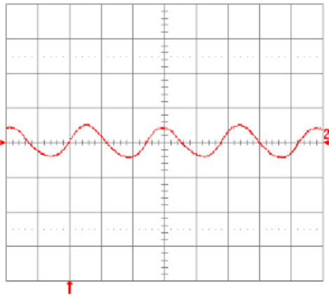
Fig. 3.3V.15: Input reflected ripple current, i_c (100 mA/div.), measured at input terminals at full rated load current and V_{in} = 48\text{V} . Refer to Fig. 3.3V.14 for test setup. Time scale: 1 \mu\text{s} /div.
