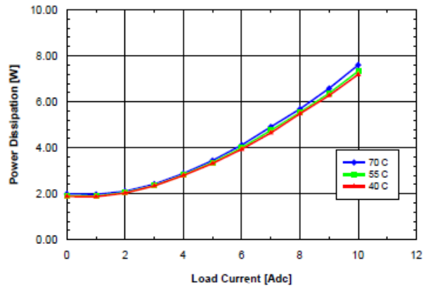
Fig. 5.0V.8: Power dissipation vs. load current and ambient temperature for SQ48T/S10050 converter mounted vertically with V_{in} = 48\text{V} and air flowing from pin 3 to pin 1 at a rate of 200LFM (1.0m/s).
