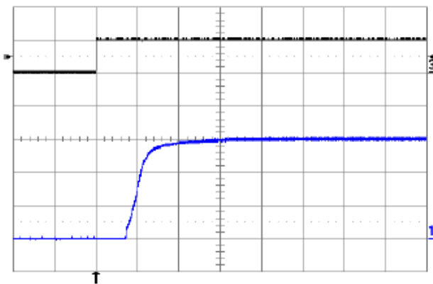
Fig. 6.0V.7: Turn-on transient at full rated load current (resistive) with no output capacitor at V_{in} = 48\text{V} , triggered via ON/OFF pin. Top trace: ON/OFF signal (5V/div.). Bottom trace: output voltage (2V/div.). Time scale: 2ms/div.
