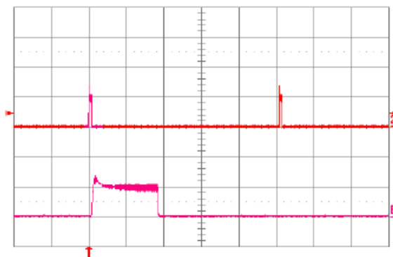
Fig. 12V.16: Load current (top trace, 5A/div., 20 ms/div.) into a 10\text{ m}\Omega short circuit during restart, at V_{in} = 48V . Bottom trace (5A/div., 1ms/div.) is an expansion of the on-time portion of the top trace.
