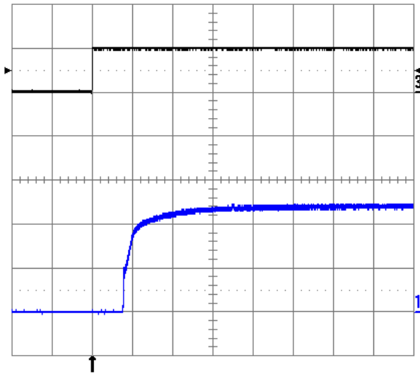
Fig. 1.2V.9: Turn-on transient at full rated load current (resistive) with no output capacitor at V_{in} = 48V , triggered via ON/OFF pin. Top trace: ON/OFF signal (5V/div.). Bottom trace: output voltage (0.5V/div.). Time scale: 2ms/div.
