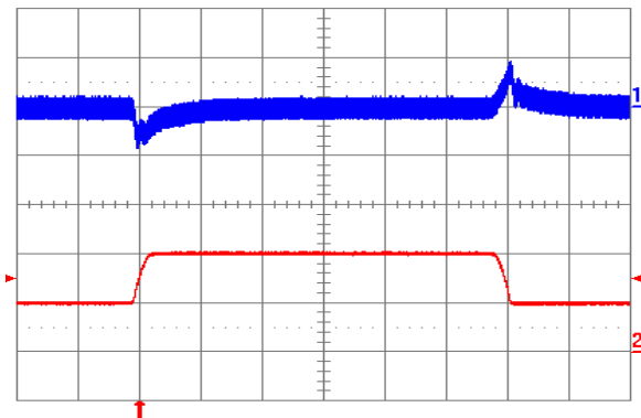
Fig. 2.5V.5: Output voltage response to load current step-change (5 A – 10 A – 5 A) at V_{in} = 48\text{ V} . Top trace: output voltage (100 mV/div.). Bottom trace: load current (5 A/div.). Current slew rate: 0.1 A/ \mu\text{s} . C_o = 1\ \mu\text{F} ceramic. Time scale: 0.2 ms/div.
