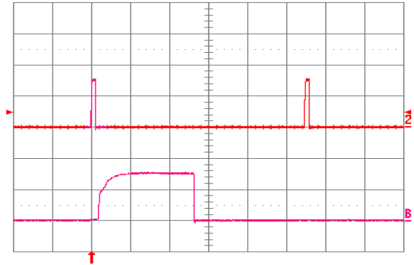
Fig. 2.5V.12: Load current (top trace, 20 A/div., 20 ms/div.) into a 10 mΩ short circuit during restart, at V in = 48 V. Bottom trace (20 A/div., 1 ms/div.) is an expansion of the on-time portion of the top trace.
