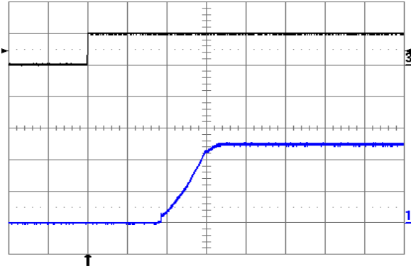
Fig. 2.5V.3: Turn-on transient at full rated load current (resistive) with no output capacitor at V_{in} = 48\text{ V} , triggered via ON/OFF pin. Top trace: ON/OFF signal (5 V/div.). Bottom trace: output voltage (1 V/div.). Time scale: 1 ms/div.
