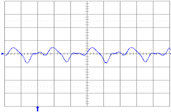
Fig. 1.2V.7: Output voltage ripple (20 mV/div.) at full rated load current into a resistive load with C_o = 10 \mu\text{F} tantalum + 1\mu\text{F} ceramic and V_{in} = 48 \text{ V} . Time scale: 1 \mu\text{s}/\text{div} .
