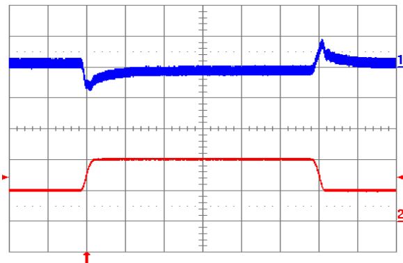
Fig. 1.8V.5: Output voltage response to load current step-change (5 A – 10 A – 5 A) at V_{in} = 48\text{ V} . Top trace: output voltage (100 mV/div.). Bottom trace: load current (5 A/div.). Current slew rate: 0.1 A/ \mu\text{s} . C_o = 1\ \mu\text{F} ceramic. Time scale: 0.2 ms/div.
