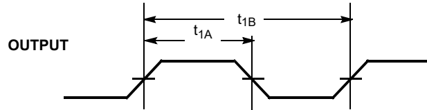
Figure 3. Duty Cycle Timing ( DC = t_{1A}/t_{1B} )
