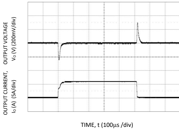
Figure 19. Transient Response to Dynamic Load Change from 0% to 50% to 0%, V_o = 0.69\text{ V}
