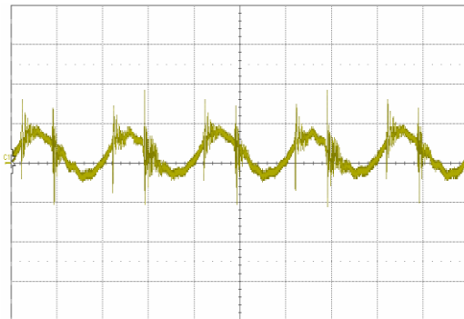
Figure 9. Output voltage ripple (20 mV/div.) at full rated load current into a resistive load with C_o = 10\mu\text{F} tantalum + 1\mu\text{F} ceramic and V_{in} =48\text{V} . Time scale: 1µs/div.
