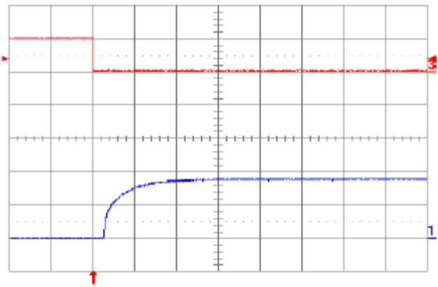
Fig. 1.8V.10: Output voltage response to load current step-change (10 A – 20 A – 10 A) at V_{in} = 48\text{ V} . Top trace: output voltage (100 mV/div.). Bottom trace: load current (10 A/div.). Current slew rate: 5 A/ \mu\text{s} . C_o = 470\ \mu\text{F} POS + 1 \mu\text{F} ceramic. Time scale: 0.2 ms/div.
