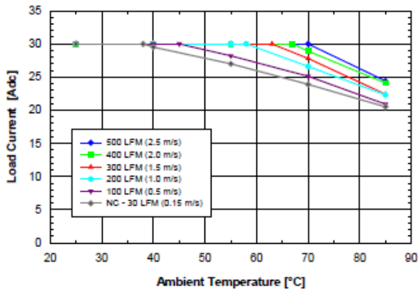
Fig. 2.5V.1: Available load current vs. ambient air temperature and airflow rates for SQE48T30025 converter mounted vertically with air flowing from pin 3 to pin 1, MOSFET temperature \leq 120 °C, Vin = 48 V.
