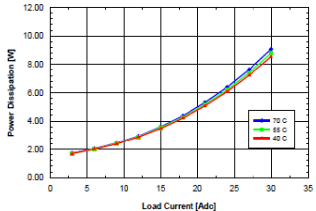
Fig. 1.8V.6: Power dissipation vs. load current and ambient temperature for SQE48T30018 converter mounted vertically with V_{in} = 48 V and air flowing from pin 3 to pin 1 at a rate of 200 LFM (1.0 m/s).
