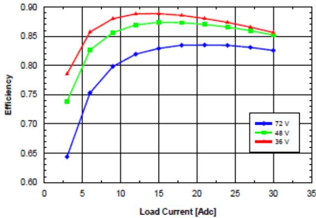
Fig. 1.5V.3: Efficiency vs. load current and input voltage for SQE48T30015 converter mounted vertically with air flowing from pin 3 to pin 1 at a rate of 300 LFM (1.5 m/s) and T_a = 25^\circ\text{C} .
