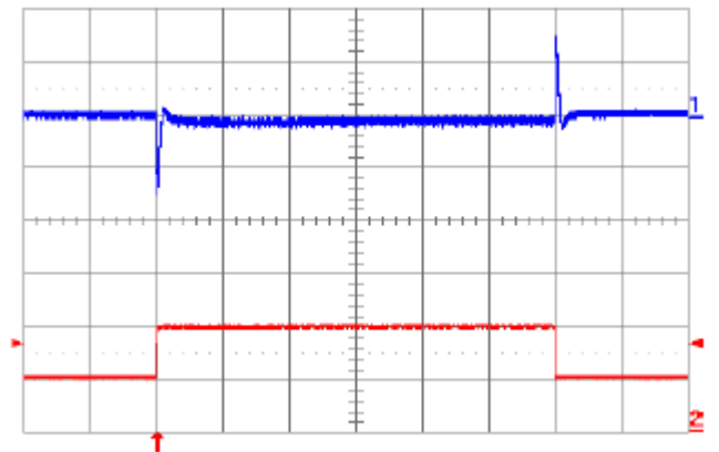
Fig. 1.8V.10: Output voltage response to load current step-change (10 A – 20 A – 10 A) at V_{in} = 48\text{ V} . Top trace: output voltage (100 mV/div.). Bottom trace: load current (10 A/div.). Current slew rate: 5 A/ \mu\text{s} . C_o = 470\ \mu\text{F} POS + 1 \mu\text{F} ceramic. Time scale: 0.2 ms/div.
