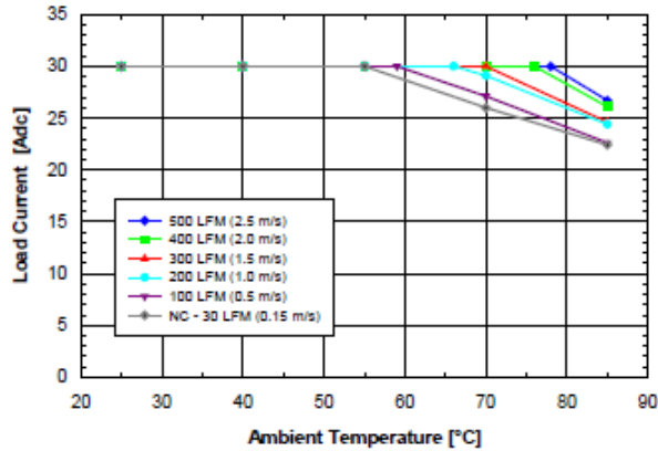
Fig. 1.8V.1: Available load current vs. ambient air temperature and airflow rates for SQE48T30018 converter mounted vertically with air flowing from pin 3 to pin 1, MOSFET temperature \leq 120 °C, V_{in} = 48 V.
