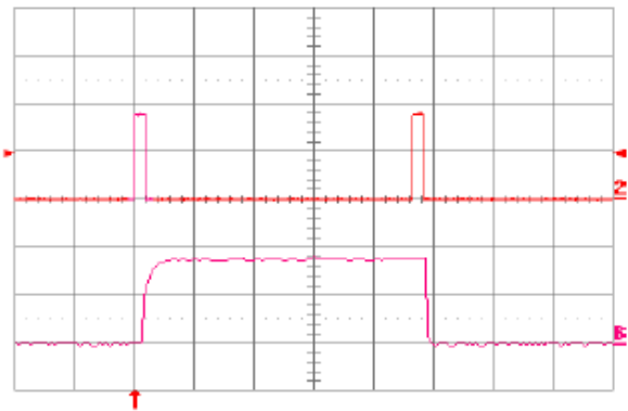
Fig. 1.5V.16: Load current (top trace, 20 A/div., 50 ms/div.) into a 10 mΩ short circuit during restart, at Vin = 48 V. Bottom trace (20 A/div., 2 ms/div.) is an expansion of the on-time portion of the top trace.
