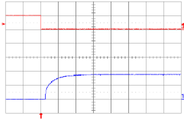
Fig. 1.8V.9: Output voltage response to load current step-change (10 A – 20 A – 10 A) at V_{in} = 48\text{ V} . Top trace: output voltage (100 mV/div.). Bottom trace: load current (10 A/div.). Current slew rate: 0.1 A/ \mu\text{s} . C_o = 1\ \mu\text{F} ceramic. Time scale: 0.2 ms/div.
