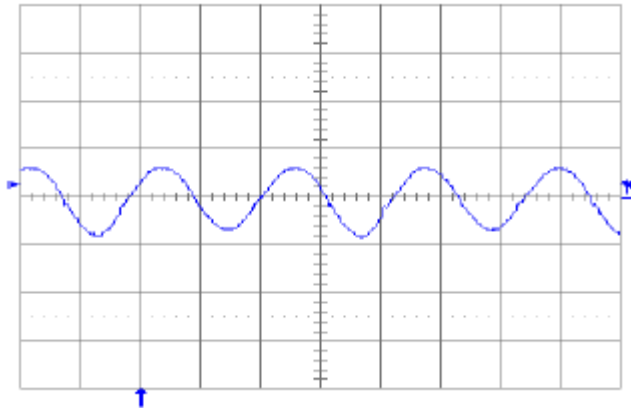
Fig. 2.5V.13: Input reflected-ripple current, i_c (100 mA/div.), measured at input terminals at full rated load current and V_{in} = 48 \text{ V} . Refer to Fig. 2.5V.12 for test setup. Time scale: 1 \mu\text{s}/\text{div} .
