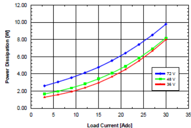
Fig. 1.8V.5: Power dissipation vs. load current and input voltage for SQE48T30018 converter mounted vertically with air flowing from pin 3 to pin 1 at a rate of 300 LFM (1.5 m/s) and T_a = 25 °C.
