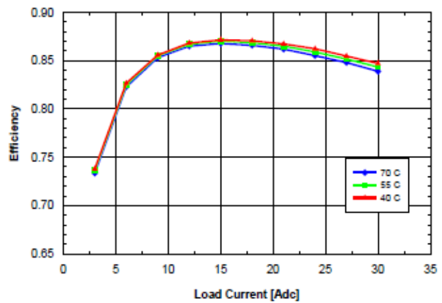
Fig. 1.5V.4: Efficiency vs. load current and ambient temperature for SQE48T30015 converter mounted vertically with V_{in} = 48\text{ V} and air flowing from pin 3 to pin 1 at a rate of 200 LFM (1.0 m/s).
