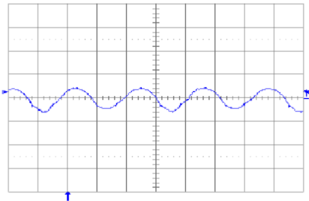
Fig. 1.8V.11: Output voltage ripple (20 mV/div.) at full rated load current into a resistive load with C_o = 10\ \mu\text{F} tantalum + 1 \mu\text{F} ceramic and V_{in} = 48\text{ V} . Time scale: 1 \mu\text{s} /div.
