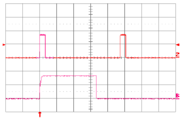
Fig. 1.2V.16: Load current (top trace, 20 A/div., 50 ms/div.) into a 10 \text{ m}\Omega short circuit during restart, at V_{in} = 48 \text{ V} . Bottom trace (20 A/div., 5 ms/div.) is an expansion of the on-time portion of the top trace.
