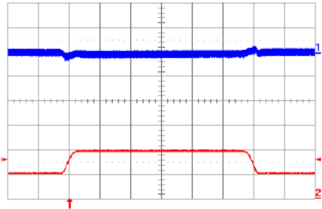
Fig. 1.8V.9: Output voltage response to load current step-change (10 A – 20 A – 10 A) at V_{in} = 48\text{ V} . Top trace: output voltage (100 mV/div.). Bottom trace: load current (10 A/div.). Current slew rate: 0.1 A/ \mu\text{s} . C_o = 1\ \mu\text{F} ceramic. Time scale: 0.2 ms/div.
