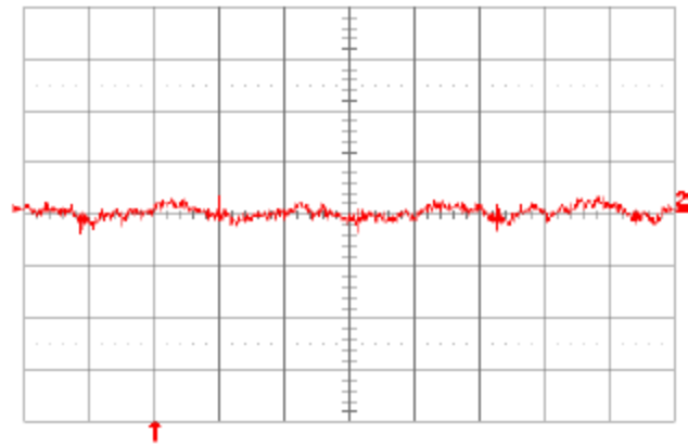
Fig. 1.2V.14: Input reflected-ripple current, i_s (10 mA/div.), measured through 10 \mu\text{H} at the source at full rated load current and V_{in} = 48 \text{ V} . Refer to Fig. 1.2V.12 for test setup. Time scale: 1 \mu\text{s}/\text{div} .
