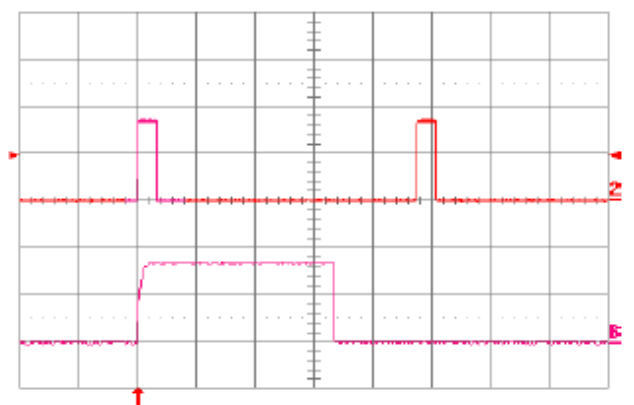
Fig. 1.2V.16: Load current (top trace, 20 A/div., 50 ms/div.) into a 10 \text{ m}\Omega short circuit during restart, at V_{in} = 48 \text{ V} . Bottom trace (20 A/div., 5 ns/div.) is an expansion of the on-time portion of the top trace.
