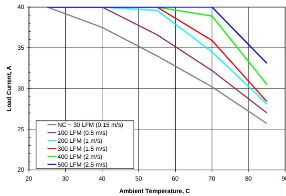
Figure 1. Available load current vs. ambient air temperature and airflow rates for SQE48T40018 converter mounted vertically with air flowing from pin 3 to pin 1, MOSFET temperature \leq 120^\circ\text{C} , V_{in} = 48\text{ V} . Note: NC – Natural convection
