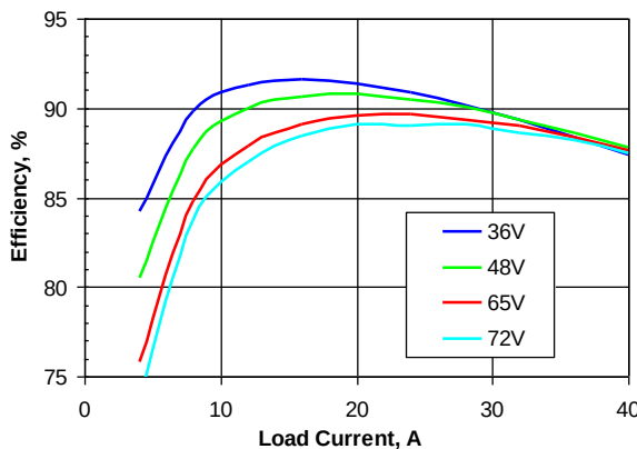
Figure 2. Efficiency vs. load current and input voltage for SQE48T40018 converter mounted vertically with air flowing from pin 3 to pin 1 at 300 LFM (1.5 m/s) and T_a=25^\circ\text{C} .
