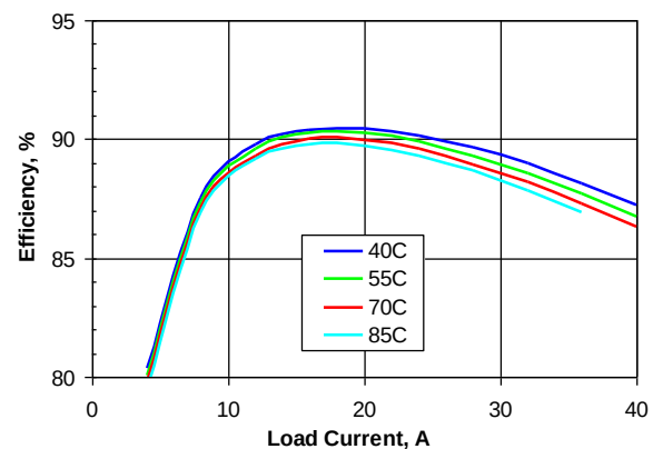
Figure 3. Efficiency vs. load current and ambient temperature for SQE48T40018 converter mounted vertically with V_{in}=48\text{V} and air flowing from pin 3 to pin 1 at 200LFM (1.0m/s).
