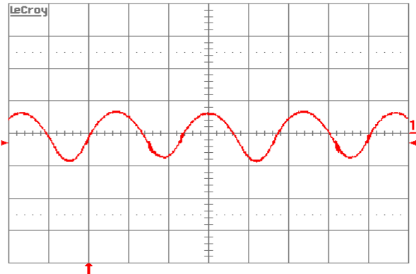
Figure 13. Input reflected ripple-current, i_C (200 mA/div.), measured at input terminals at full rated load current and V_{in} = 48\ \text{V} . Refer to Figure 11 for test setup. Time scale: 1\ \mu\text{s}/\text{div} .
