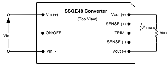
Fig. C: Configuration for increasing output voltage.
