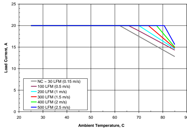
Figure 1: Available load current vs. ambient air temperature and airflow rates for SSQE48T20033 converter mounted vertically with air flowing from pin 1 to pin 3, V_{in} = 48\text{V} . Note: NC – Natural convection
