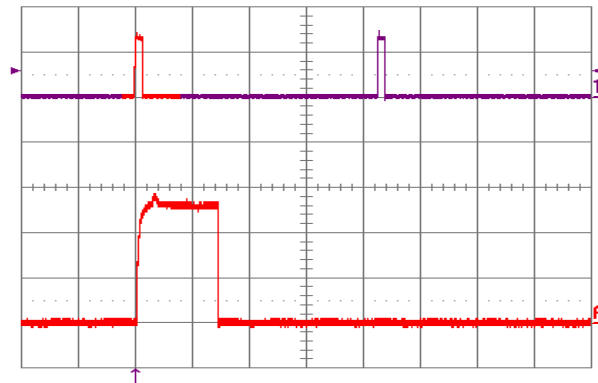
Figure 15: Load current (top trace, 20 \text{ A}/\text{div} ., 50 \text{ ns}/\text{div} .) into a 10 \text{ m}\Omega short circuit during restart, at V_{in} = 48 \text{ V} . Bottom trace ( 10 \text{ A}/\text{div} ., 5 \text{ ns}/\text{div} .) is an expansion of the on-time portion of the top trace.
