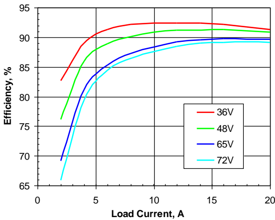
Figure 2: Efficiency vs. load current and input voltage for SSQE48T20033 converter mounted vertically with air flowing from pin 1 to pin 3 at a rate of 300 LFM (1.5 m/s) and T_a=25^\circ\text{C} .
