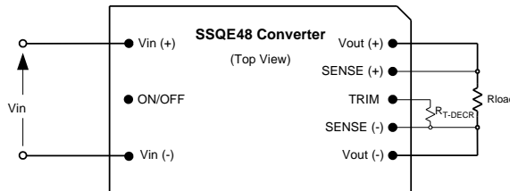
Fig. D: Configuration for decreasing output voltage
