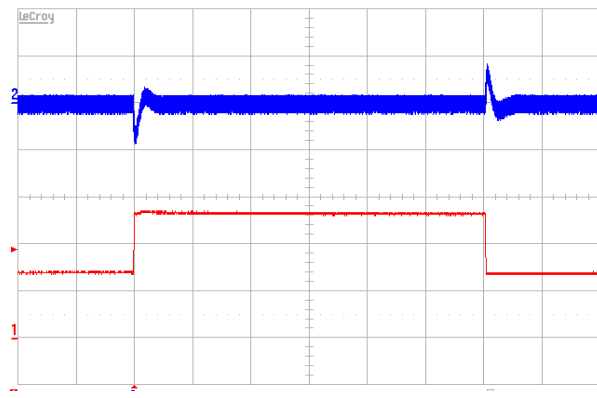
Figure 9. Output voltage response to load current step-change (3.5 A-5.25 A-3.5 A) at V_{in} = 48\text{ V} . Top trace: V_{out} (100 mV/div.). Bottom trace: I_{out} (2 A/div.), Time: (0.2 ms/div.) Current slew rate: 5 A/ \mu\text{s} . C_o = 470\text{ }\mu\text{F} POS + 1 \mu\text{F} ceramic.
