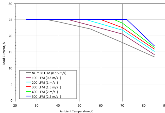
Figure 1. Available load current vs. ambient air temperature and airflow rates for SSQE48T25025 converter mounted vertically with air flowing from pin 1 to pin 3, V_{in} = 48V . Note: NC – Natural convection
