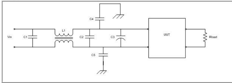
Figure 17. Typical input EMI filter circuit to attenuate conducted emissions.
