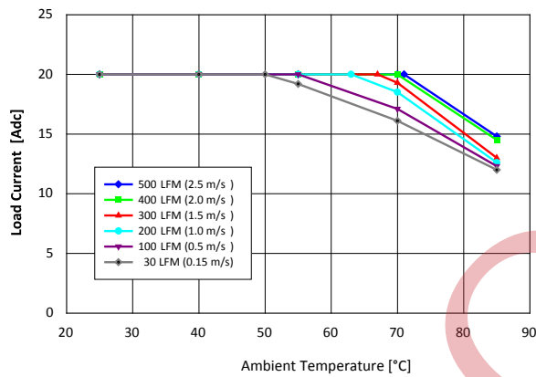
Figure 1. Available load current vs. ambient air temperature and airflow rates for SSQL48T20033 converter mounted vertically with air flowing from pin 3 to pin 1, T_C temperatures \leq 120^\circ\text{C} , V_{in} = 48\text{ V} .
