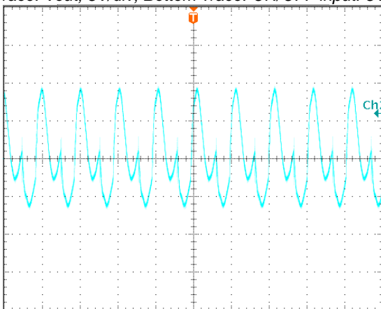
Output voltage ripple at nominal input voltage and max load current (10mV/div, 2µs/div) Load cap: 10µF, tantalum capacitor and 1µF ceramic capacitor. Bandwidth: 20MHz.
