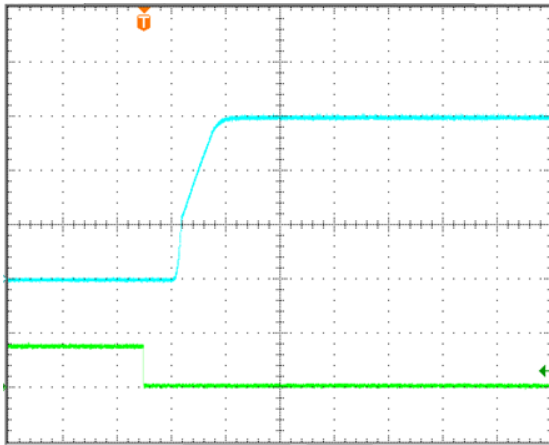
Turn-on transient at full load current (10ms/div). Top Trace: Vout; 5V/div; Bottom Trace: ON/OFF input; 5V/div.
