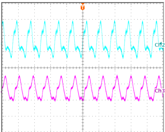
Output voltage ripple at nominal input voltage and max load current Top trace +12V, 10 mV/div, Bottom trace -12V, 20mV/div, 2us/div. Load cap: 10 \mu F, tantalum capacitor and 1 \mu F ceramic capacitor. Bandwidth: 20 MHz.
