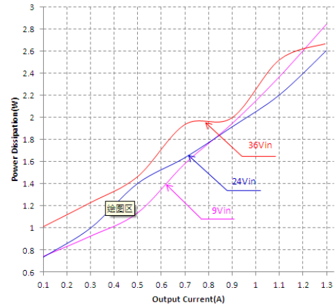
Power dissipation vs. load current at 25°C.
