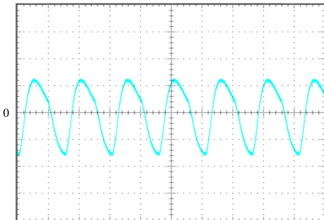
Output voltage ripple at nominal input voltage and max load current (20mV/div, 2µs/div) Load cap: 10µF, tantalum capacitor and 1µF ceramic capacitor. Bandwidth: 20MHz.
