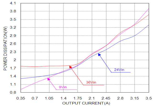
Power dissipation vs. load current at 25°C.
