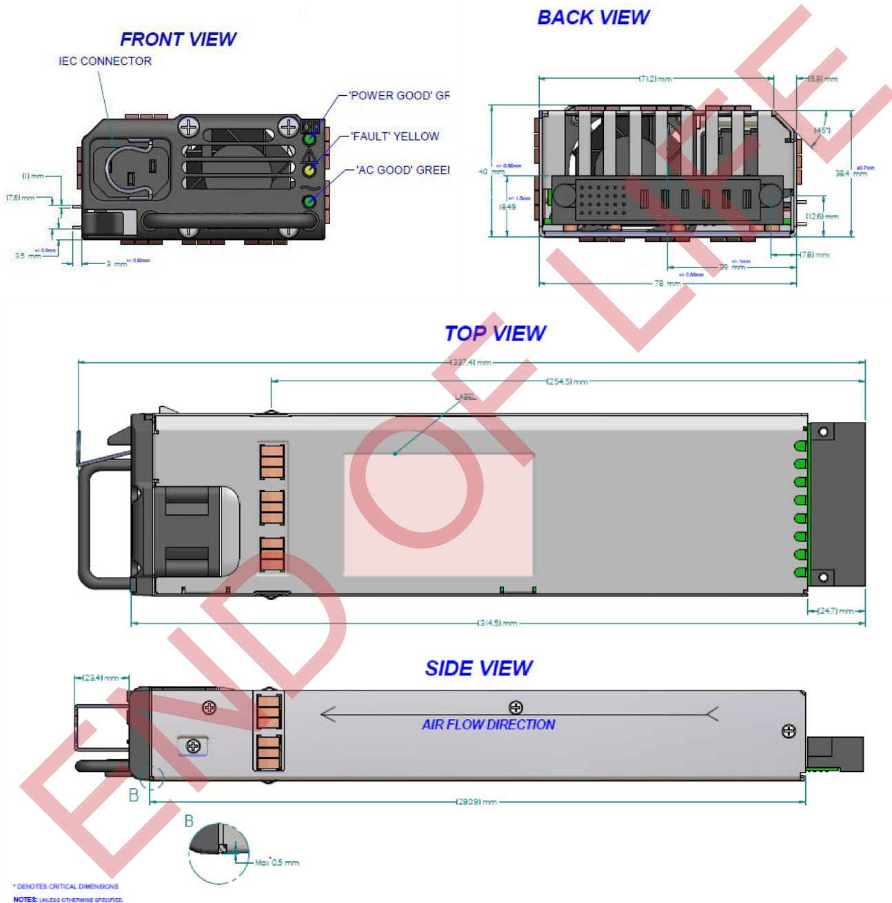
Figure 1. Mechanical Drawings
