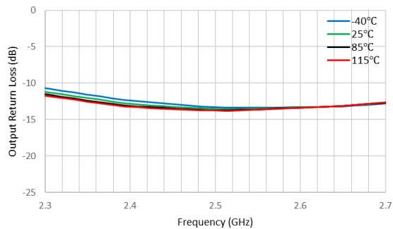
Figure 34. Output Return Loss (dB) vs Frequency
