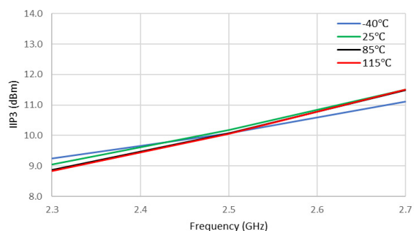
Figure 36. IIP3 (dBm) vs Frequency (GHz)
