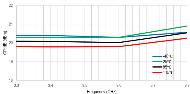
Figure 24. OP1dB (dBm) vs Frequency (GHz)
