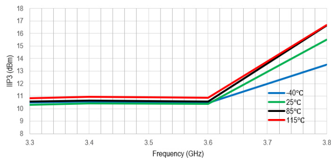
Figure 22. IIP3 (dBm) vs Frequency (GHz)
