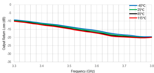
Figure 20. Output Return Loss (dB) vs Frequency (GHz)
