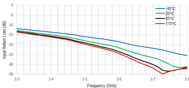
Figure 19. Input Return Loss (dB) vs Frequency (GHz)
