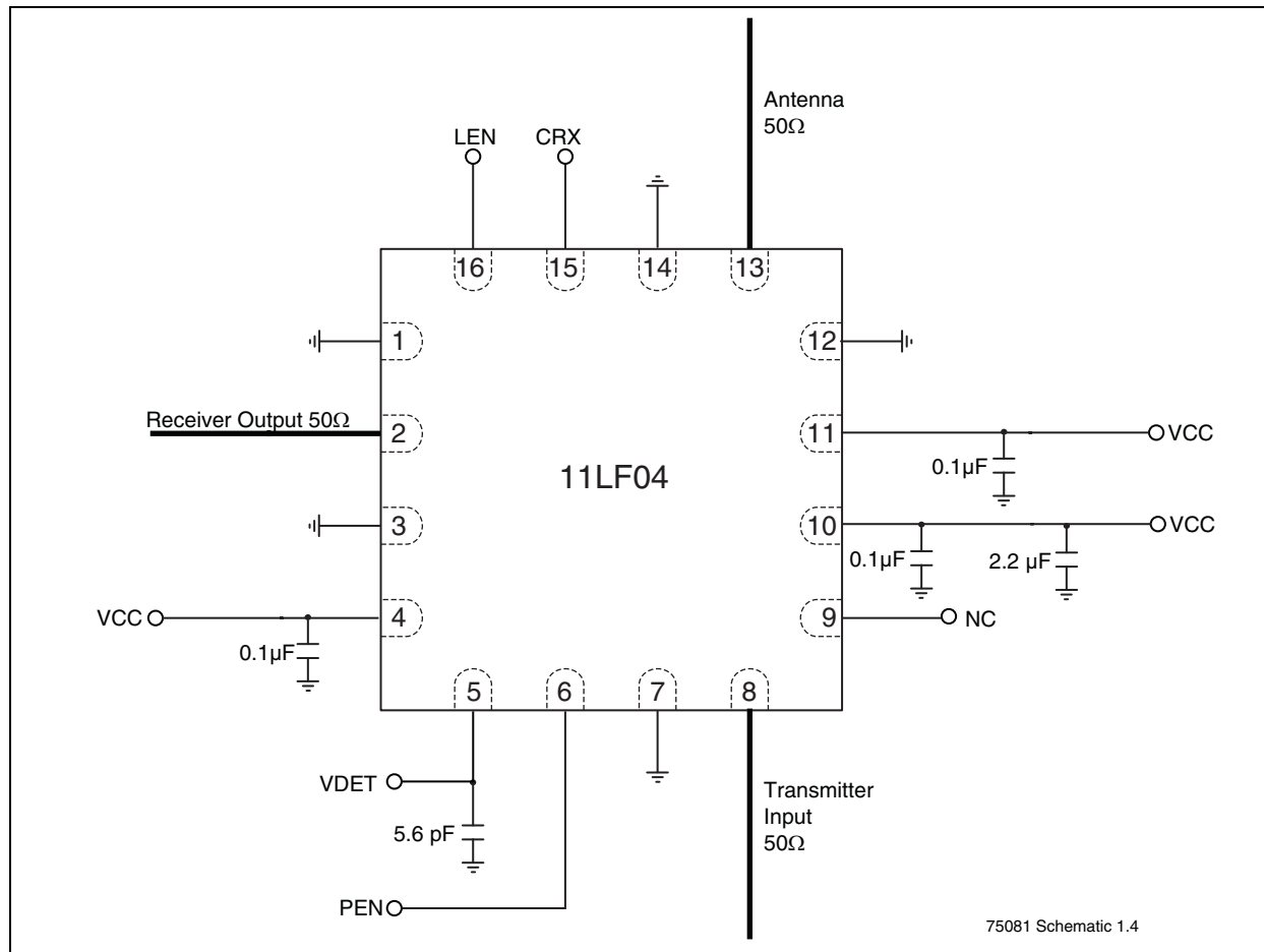
FIGURE 6-1: TYPICAL SCHEMATIC
