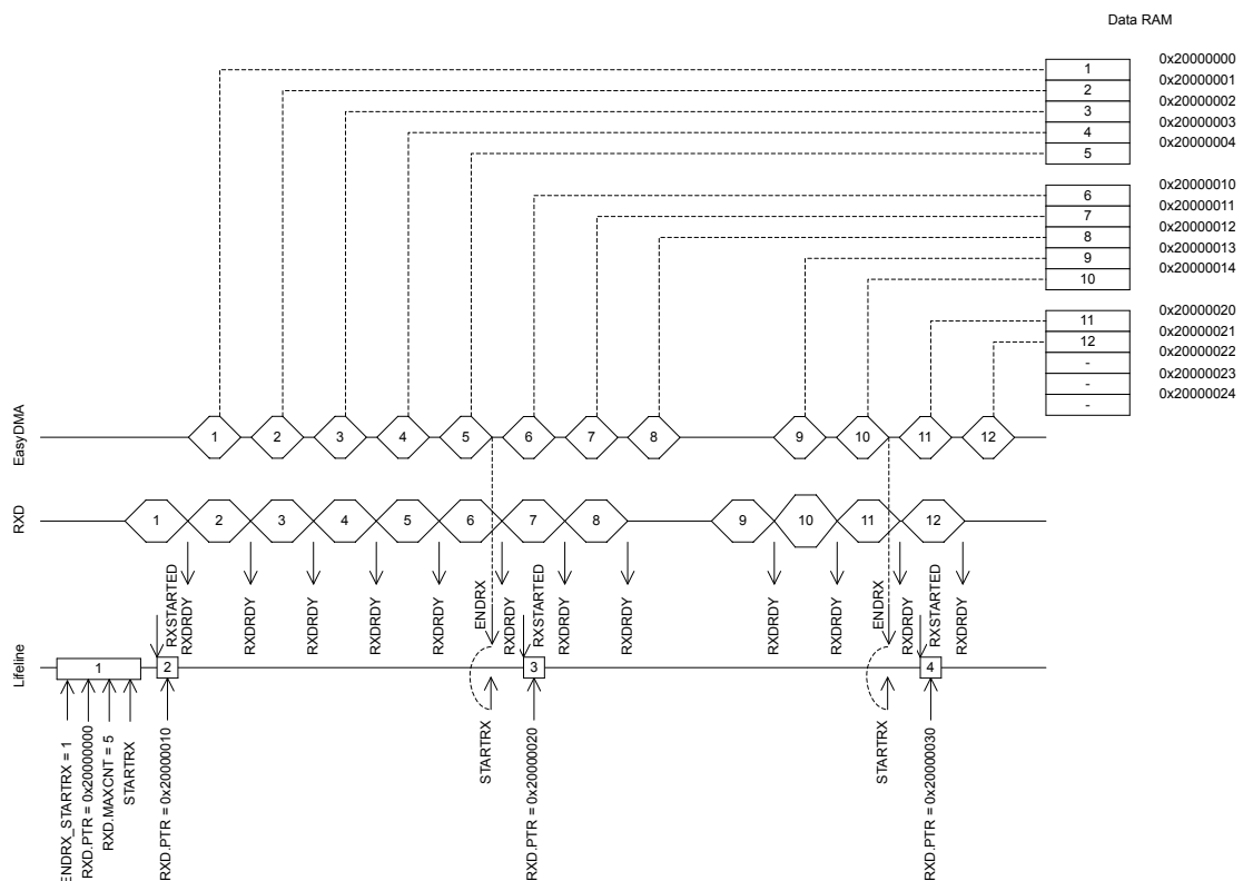
Figure 115: UARTE reception
