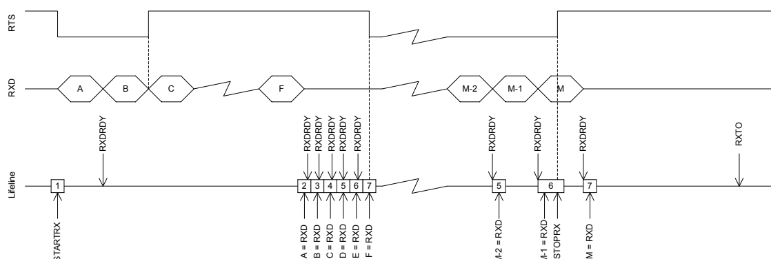
Figure 112: UART reception
