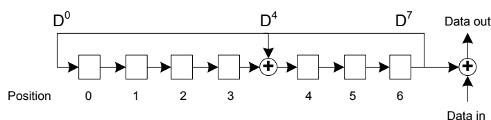
Figure 40: Data whitening and de-whitening
