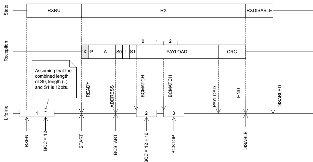
Figure 50: Bit counter example
