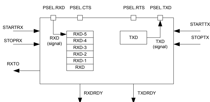
Figure 110: UART configuration
