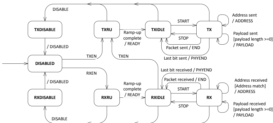
Figure 42: Radio states
