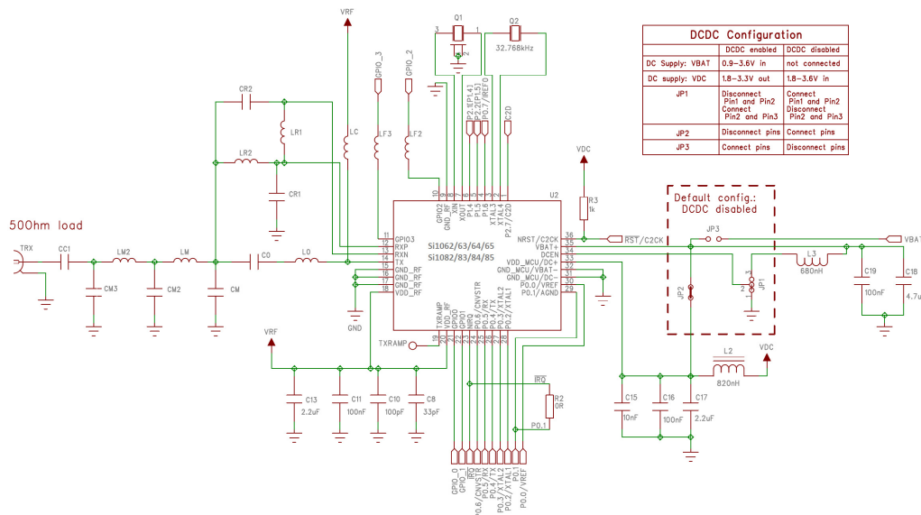
Figure 1.2. Si106x/108x RX/TX Direct-Tie Application Example
