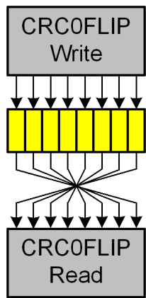
Figure 14.2. Bit Reverse Register
