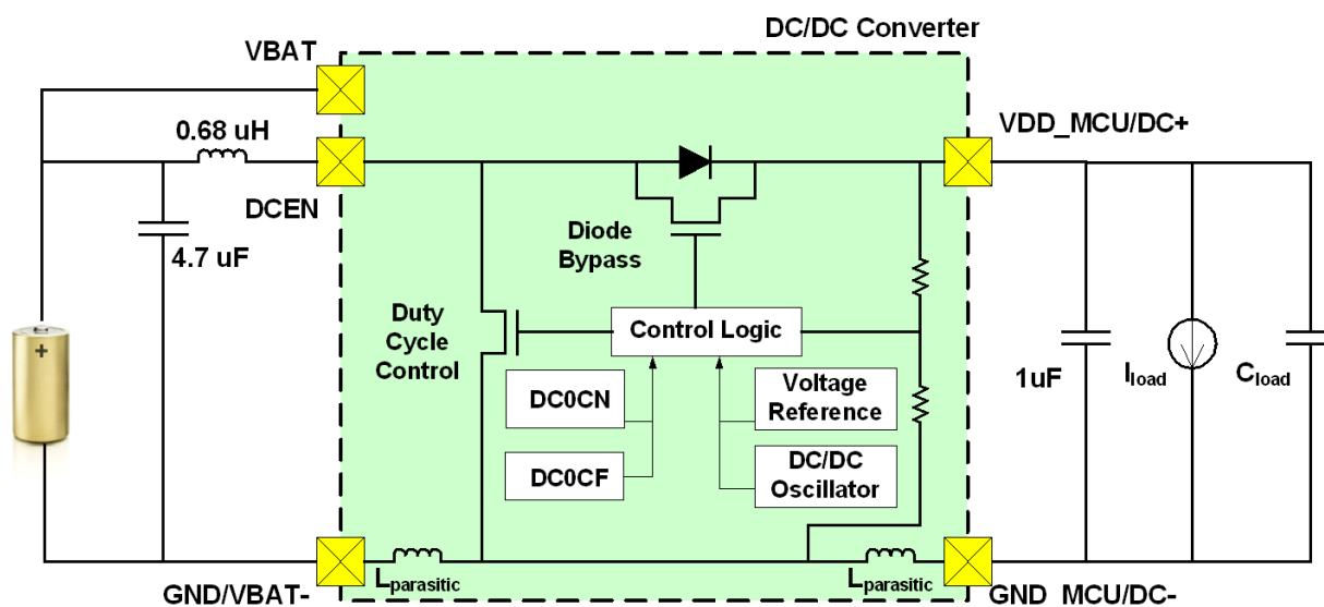
Figure 15.1. DC-DC Converter Block Diagram
