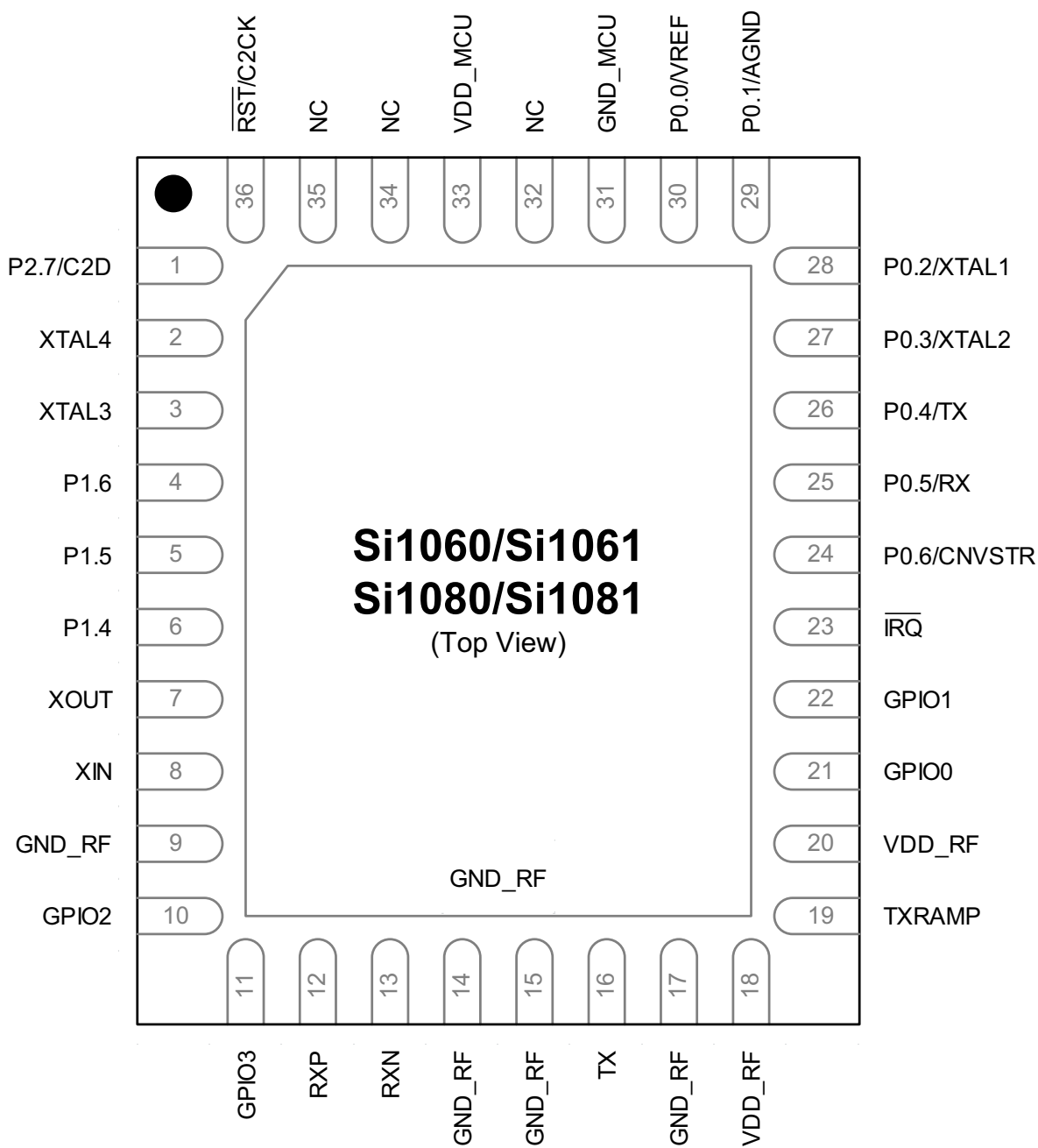
Figure 3.1. Si1060/1, Si1080/1-A-GM Pinout Diagram (Top View)
