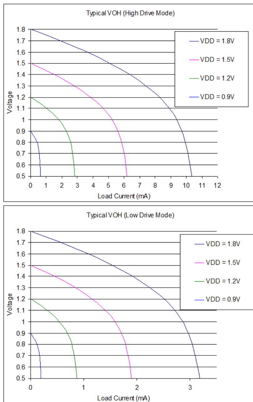
Figure 4.8. Typical V_{OH} Curves, 0.9–1.8 V
