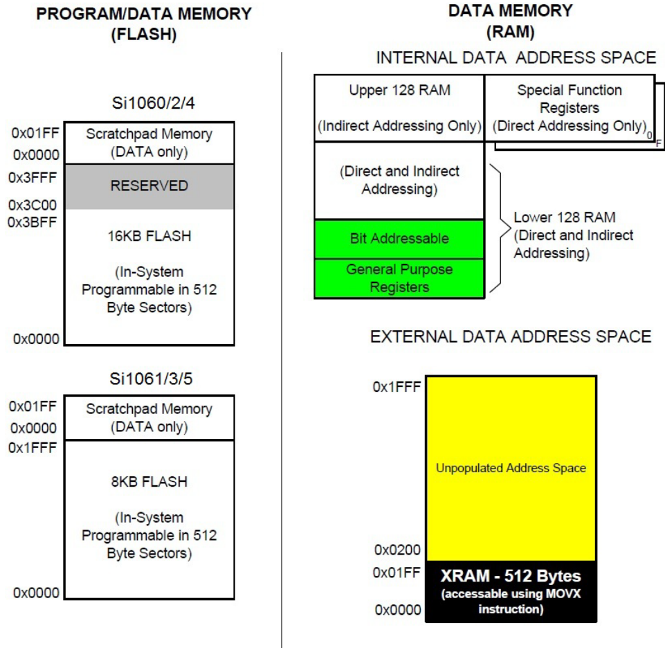
Figure 8.2. Si108x Memory Map
