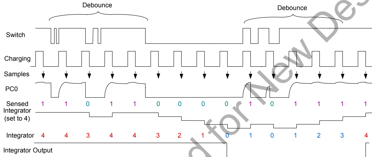
Figure 25.4. Debounce Timing
