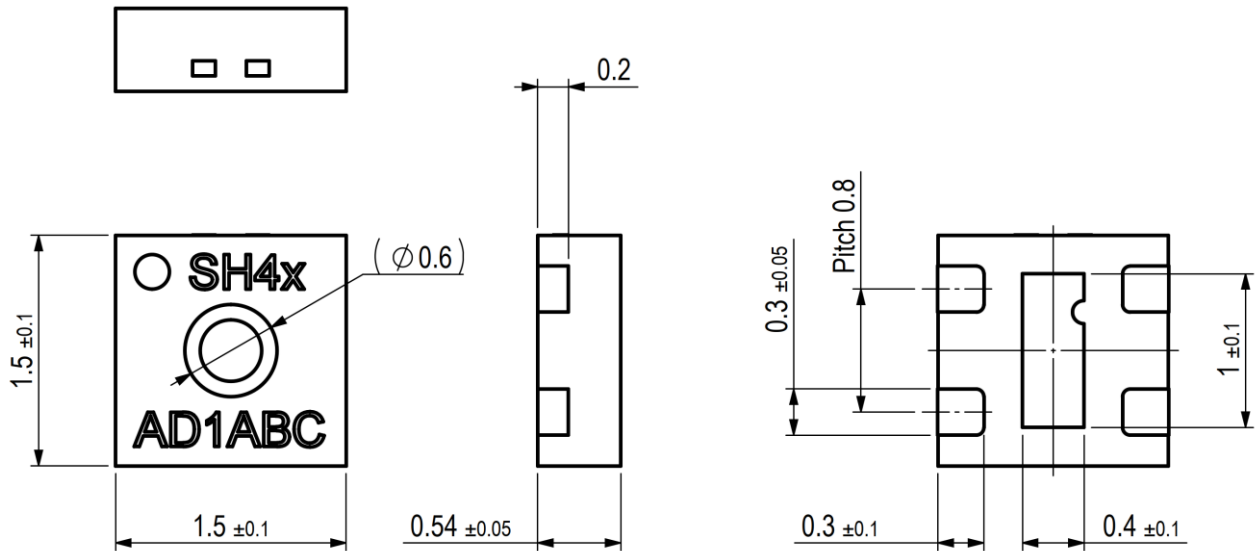
Figure 9 Dimensional drawing of SHT4x including package tolerances (units mm).
