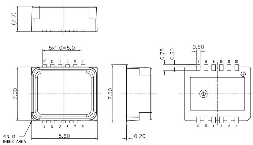
Figure 2. Housing dimensions
