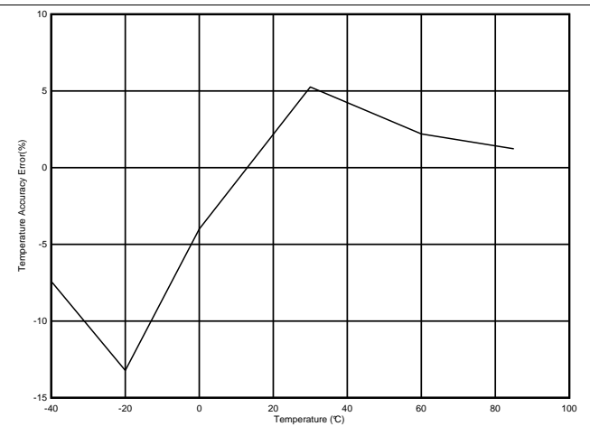
Figure 4. Temperature Accuracy
