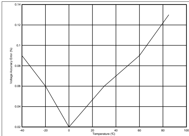
Figure 3. Voltage Accuracy
