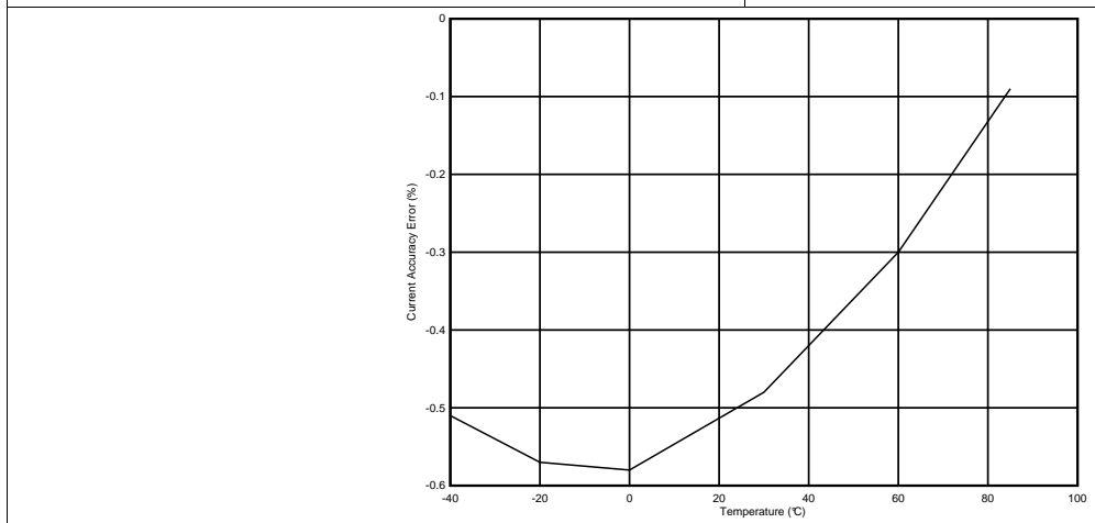
Figure 5. Current Accuracy
