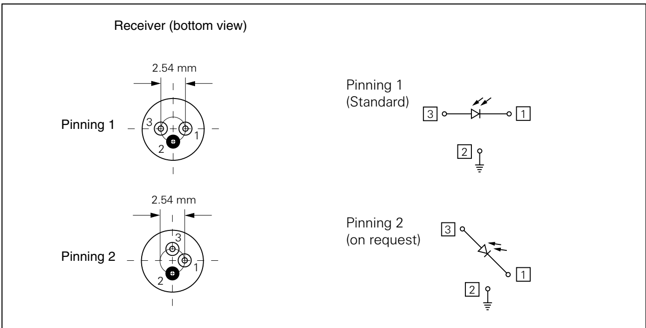
Figure 2 Receiver
